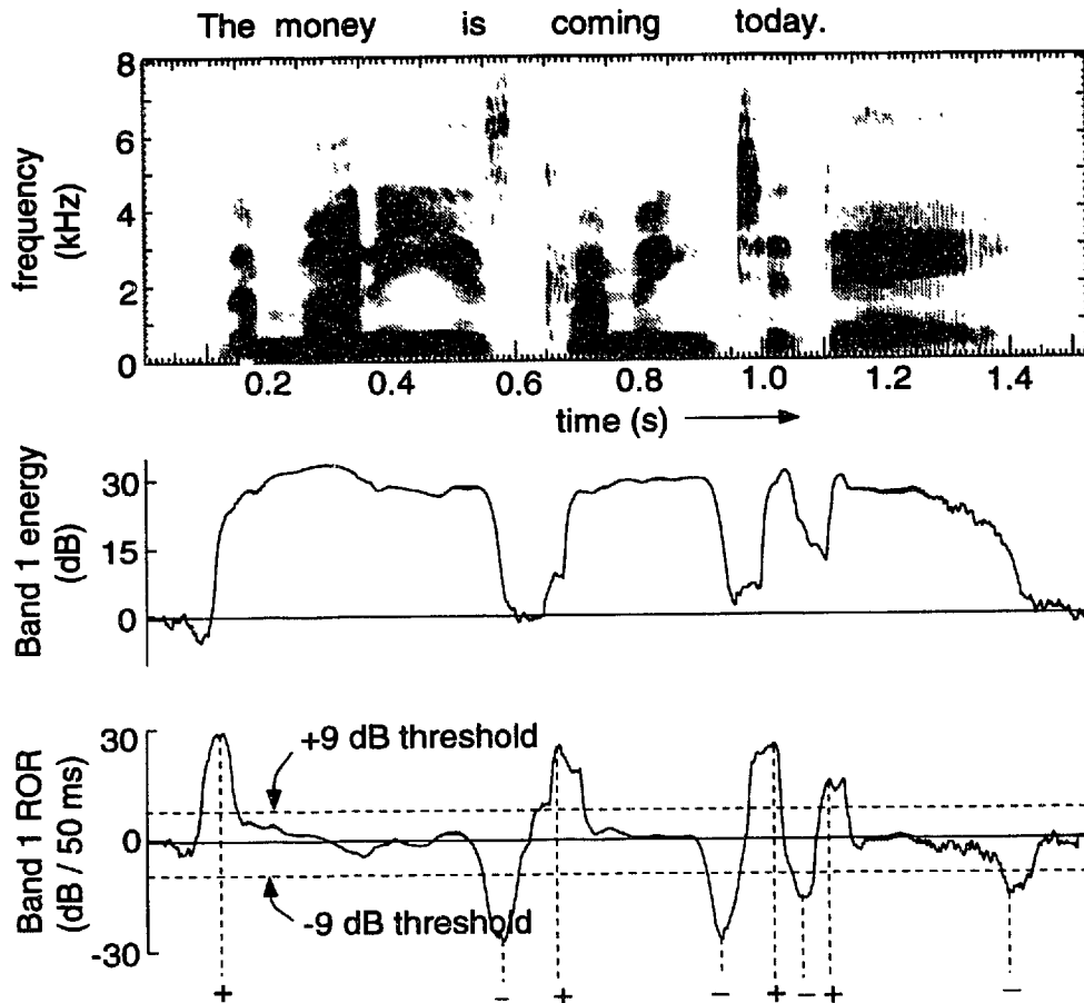
Figure 3.3: An illustration of general processing. The top panel shows a spectrogram for the utterance “The money is coming today”. The middle panel is the Band 1 energy and the bottom panel is the Band 1 ROR, both from coarse processing. The two dotted horizontal lines are thresholds for peak picking. The peaks detected are shown with \pm signs indicating the polarity of the peaks. Band 1 peaks are also likely candidates for g(lottis) landmarks.
