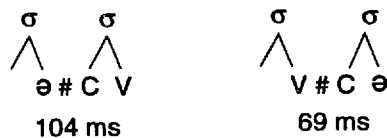
Figure 3.8: The effect of vowel reduction and syllable affiliation on consonant duration.
