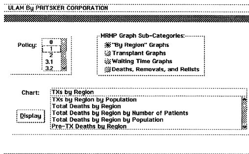
Figure 3: OUTPUT-MRMP Screen of ULAM User Interface
