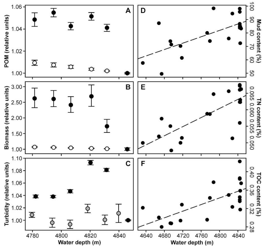
Figure 2. Terrain elevation related variations in megafauna biomass and organic matter supply terms. (A) Particulate organic matter (POM) seabed cover (observed mean \bullet and 95% confidence interval; null prediction \circ and 95% CI). (B) Megafauna biomass (observed mean \bullet and 95% CI; null prediction \circ and 95% CI). (C) Turbidity in water column (altitude >10 m, \bullet ), and benthic boundary layer (altitude <10 m, \bullet ), as mean and 95% CI. (A–C) Values plotted normalised to the abyssal plain (plain value = 1.00). (D) Sediment mud content (particles <63\mu\text{m} , 0–10 mm sediment horizon). (E) Sediment total nitrogen content (TN, 0–10 mm horizon). (F) Sediment total organic carbon content (TOC, 0–10 mm horizon). (D–F) Dashed line represents simple least squares linear fit, all relationships are significant (Spearman's rank correlation p < 0.02 ).
