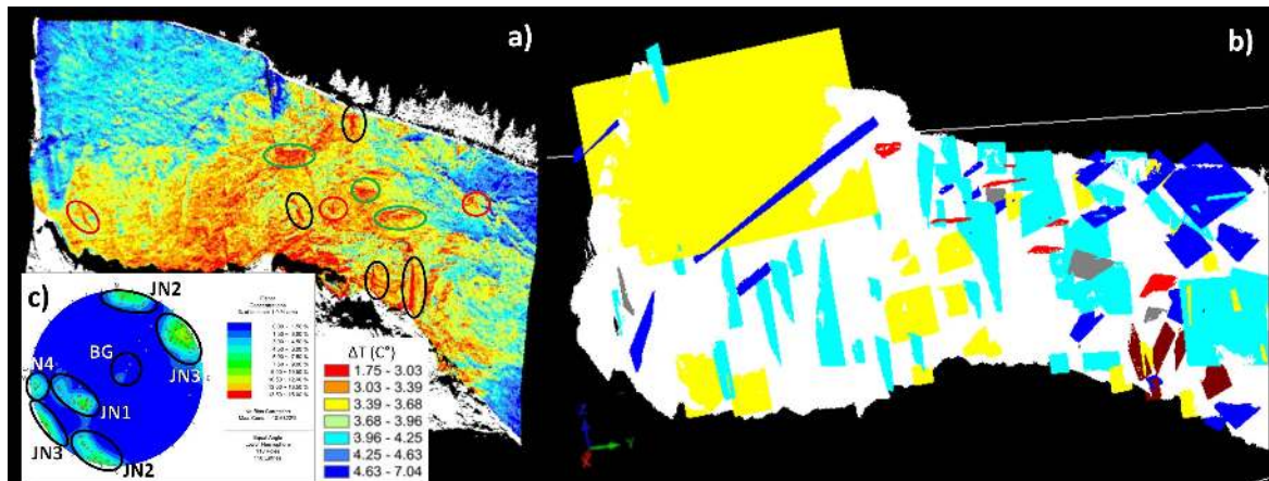
Figure 13. 3D differential surface temperature map highlighting open fractures (black ovals), niches (red ovals) and overhangs (green ovals) (a); manual extraction of discontinuity set on high resolution 3D surface (b) and resulting stereographic projection (c).
