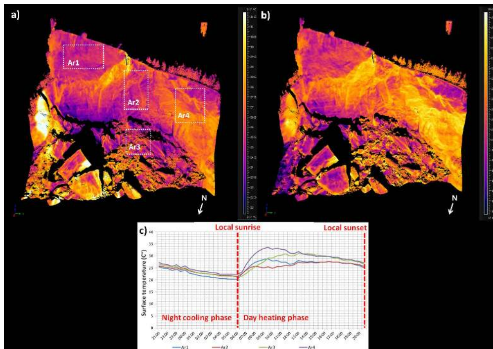
Figure 12. 3D surface temperature maps of the San Leo rock cliff: 11 June 2014, h 20:30 (a), 12 June 2014, h 05:00 (b), graph showing the 24 h average surface temperature evolution of different rock cliff sectors (Ar1: sound rock; Ar2; Ar4: intensively fractured sectors; Ar3 rock fall deposits) (c).
