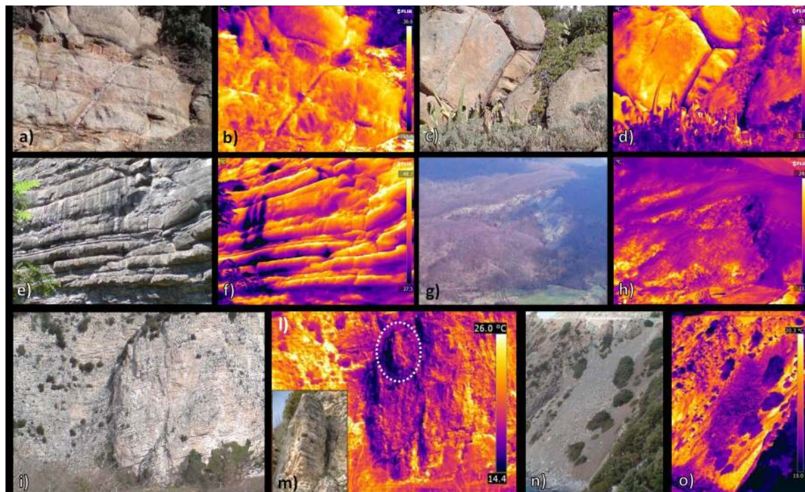
Figure 3. Examples of thermograms displaying thermal anomalies connected to slope instability phenomena in Italy. Dykelets and open fractures at Giglio Island, Tuscany (a–d); water seepage in sandstone layers (Fiesole, Tuscany) (e,f); aerial imaging of large landslide (San Benedetto Val di Sambro, Emilia Romagna) (g,h); unstable rock wall sector in (Val Nerina, Umbria) (i–m); debris apron along coastal cliff (Elba Island, Tuscany) (n,o).
