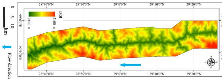
Figure 4. The digital elevation model of reservoir in Xulong hydropower station.
