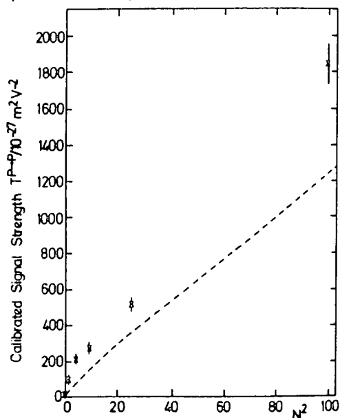
Figure 3 T^{P \rightarrow P} ( \times 10^{-27} m^2 V^{-2} ) second harmonic signal from structure shown in figure 2c plotted against the square of the number of bilayers. Dashed curve represents theoretical signal (see text)
