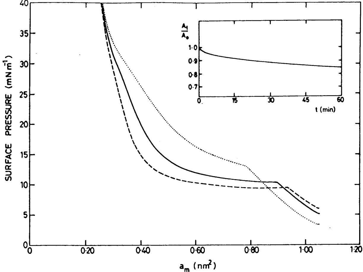
Figure 5.10 Pressure-area isotherms for D2, 2 \times 10^{-4} M \text{CdCl}_2 subphase, pH=5.7, for different periods, t , of solvent evaporation. (i) t=2 mins (----), (ii) t=4 mins (—), (iii) t=10 mins (....). Inset: Change in fractional area of D2 monolayer with time ( \pi=40 \text{ mN m}^{-1} , pH=5.8, 2 \times 10^{-4} M \text{CdCl}_2 ).
