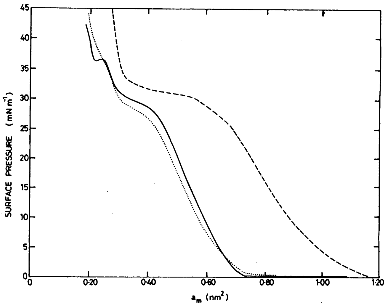
Figure 5.9 Pressure-area isotherms for D1 (i) D1A ( \text{pH}=7.6 , 10^{-3} \text{ M (NH}_4)_2\text{SO}_4 ) (----), (ii) D1B ( \text{pH}=7.4 , no ions) under slow (—) and rapid (....) compression.
