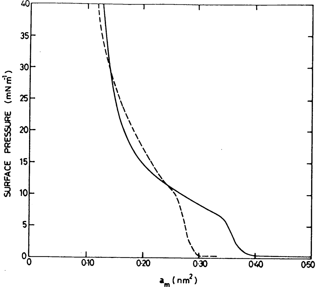
Figure 5.8 Pressure-area isotherms for A8 (—) and A9 (----), on a 2 \times 10^{-4} \text{ M CdCl}_2 subphase, \text{pH}=5.5 .
