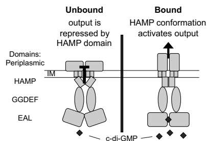
Fig. 6. A model for inside-out signaling through LapD. ( Left ) In the absence of c-di-GMP binding, the periplasmic output is repressed via the HAMP domain. ( Right ) When c-di-GMP is bound by LapD, the HAMP domain assumes a conformation that activates output. LapD is depicted as a dimer, because other HAMP domain proteins are known to be dimers.
