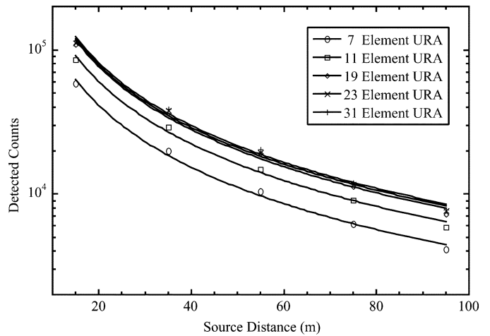
Fig. 7. Detected counts versus source distance of closest approach for different fields of view as represented by the number of pixels in the image. The curves for the largest three images are almost coincident. Note that to limit statistical noise, a simulated source strength of 10 mCi was used.
