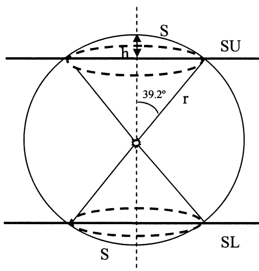
Fig. 1. Scintillation light originating in point 0 can escape from the scintillator in a cone limited by total reflection angle 39.2^\circ (refractive index 1.58). 0 – origin of scintillation; r – radius; S – cap surface; h – height of cap; SU – scintillator upper plane; SL – scintillator lower plane.
