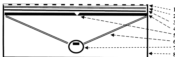
Fig. 2. Layout of the scintillation probe. 1 – protection grid; 2 – three layers of aluminized foil; 3 – ZnS(Ag) phosphor on a thin plastic foil; 4 – plastic scintillator 250 \times 125 \times 1 mm 3 ; 5 – intersection of plastic scintillator; 6 – light reflector; 7 – side window PMT; 8 – light tight housing.
