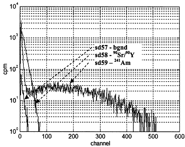
Fig. 4. Differential spectra of background, ^{90}\text{Sr}/^{90}\text{Y} and ^{241}\text{Am} measured with a Genie 2000 multichannel analyzer.
