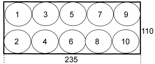
Fig. 5. Placement of measured positions of scintillation probe. Dimensions of active area of the scintillator are given in mm.
