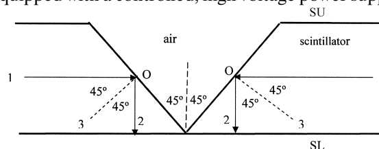
Fig. 3. The path of internal reflection of scintillation light inside the scintillator. 0–1 – incident light at 45^\circ cut scintillator edge; 0–2 – reflected light; 3–0 – normal line; SU – scintillator upper plane; SL – scintillator lower plane.
