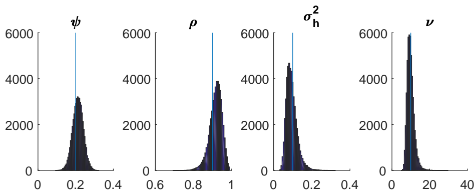
Figure 6: Histograms of the posterior draws of \psi , \rho , \sigma_h^2 and \nu . The true values are represented by the solid lines.
