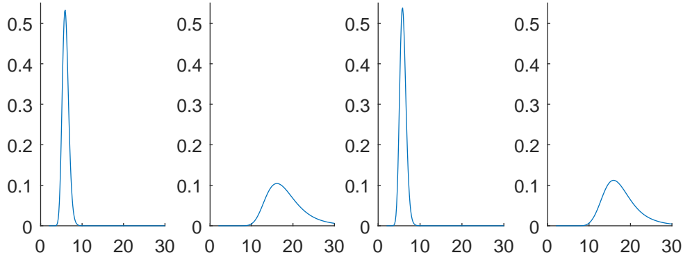
Figure 5: Posterior densities of the degree of freedom parameter \nu under (from left to right) BVAR- t , BVAR- t -CSV, BVAR- t -MA, and BVAR- t -CSV-MA.
