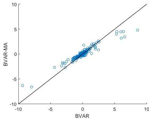
Figure 3: Scatter plot of VAR coefficients under BVAR-MA against BVAR.
