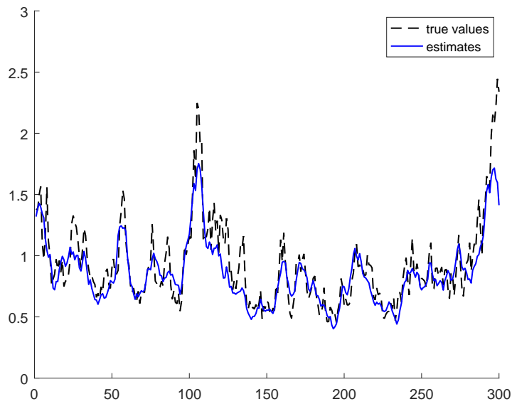
Figure 8: Posterior estimates and the true values of \exp(h_t/2) .
