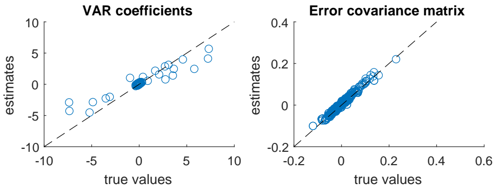
Figure 7: Posterior estimates and the true parameter values of the VAR coefficients and the unique elements in the covariance matrix.
