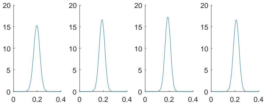
Figure 2: Posterior densities of the MA(1) coefficient \psi under (from left to right) BVAR-MA, BVAR- t -MA, BVAR-CSV-MA, and BVAR- t -CSV-MA.
