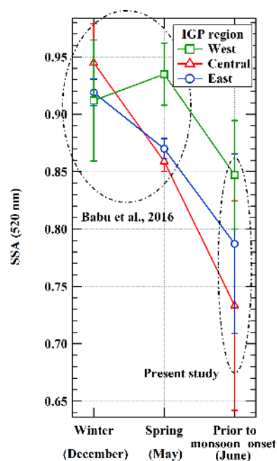
Figure 6. Seasonal variation of columnar (500–3000 m) SSA over different regions of the IGP: western (square), central (triangle) and eastern (circle). Values in the upper-left circle are calculated from Babu et al. (2016).
