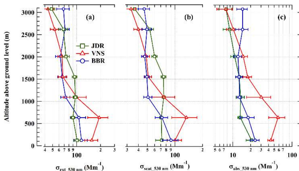
Figure 3. Mean altitudinal variation of (a) \sigma_{\text{ext}} , (b) \sigma_{\text{scat}} and (c) \sigma_{\text{abs}} over JDR (square), VNS (triangle) and BBR (circle) in logarithmic scale. Error bars represent the corresponding standard errors (standard deviation of the mean).
