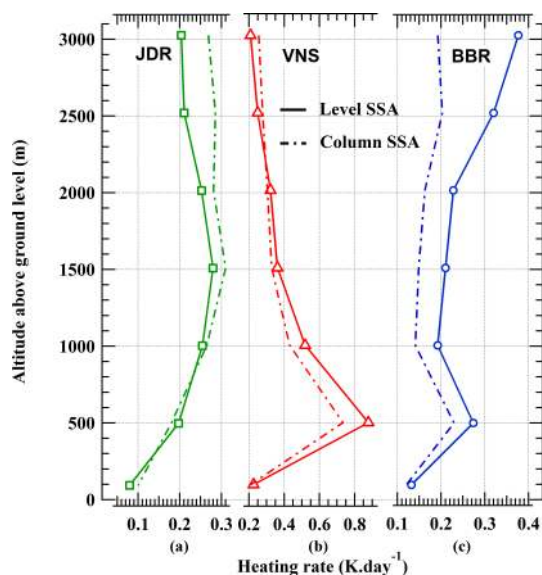
Figure 9. Altitudinal heating rate profiles for the stations (a) JDR, (b) VNS and (c) BBR. Solid lines are for heating profiles calculated using in situ aircraft profile data and layer-averaged aerosol properties. Dashed-dotted lines represent heating profiles calculated using in situ aircraft profile data and column-averaged aerosol SSA.
