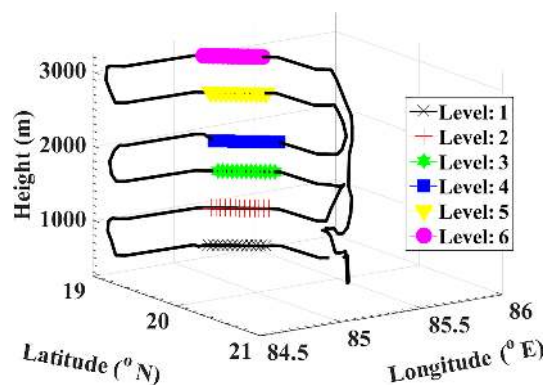
Figure 2. Typical course of the aircraft during a campaign sortie. Symbols represent stable levels. Each stable level represents a minimum of 20 min of scientifically useful measurements.
