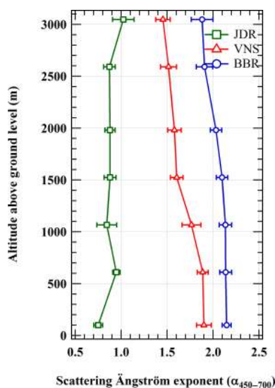
Figure 4. Altitudinal variation of \alpha for the aircraft campaign stations: JDR (square), VNS (triangle) and BBR (circle). Error bars represent the standard error in the mean of level-averaged \alpha .
