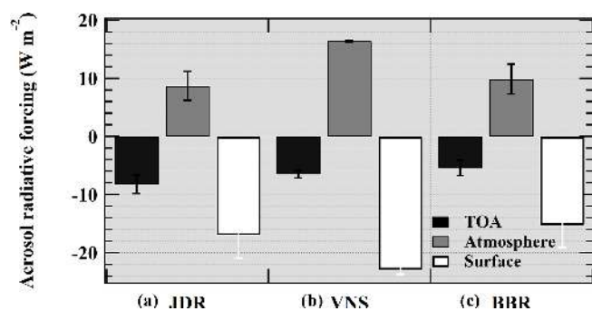
Figure 8. Aerosol-induced short-wave radiative forcing at the top of atmosphere (TOA) (filled black bar), surface (filled white bar) and atmosphere (filled grey bar) for the regions of the IGP: (a) west (JDR), (b) centre (VNS), (c) and east (BBR). Error bars represent standard deviation around the mean.
