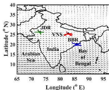
Figure 1. Geographical location of the aircraft campaign stations (solid circle) in the Indo-Gangetic Plain superimposed on the mean wind field at 850 hPa during the campaign period. JDR, VNS and BBR stand for Jodhpur, Varanasi and Bhubaneswar. Daily flight tracks are superimposed on the stations JDR (green), VNS (red) and BBR (blue) from left to right. Each measurement track has a horizontal span of \sim 150 km from the base station.
