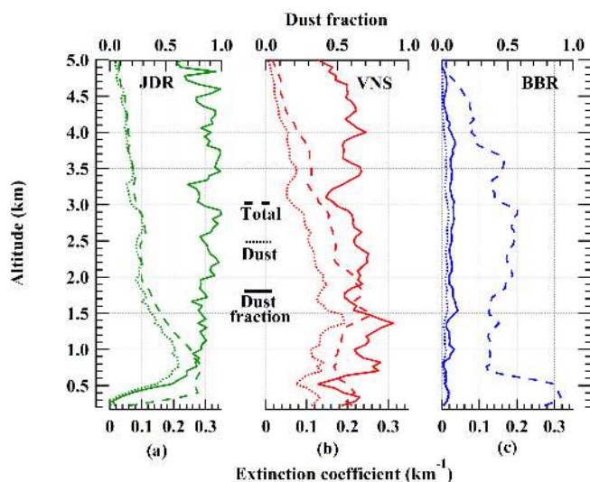
Figure 7. CALIPSO-derived total (dashed line) and dust (dotted line) extinction profiles over the stations (a) JDR, (b) VNS and (c) BBR. Also shown is the dust fraction (solid line) for the three stations.
