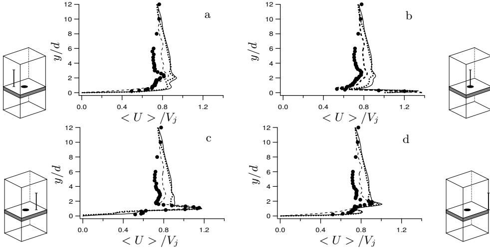
FIGURE 4. Time-averaged streamwise velocity profiles at four locations: comparison between experimental results ( \bullet ), Run A ( - - - ), Run B ( — ) and Run C ( ····· ). Graphs correspond to the locations (a), (b), (c) and (d) presented in figure 9.
