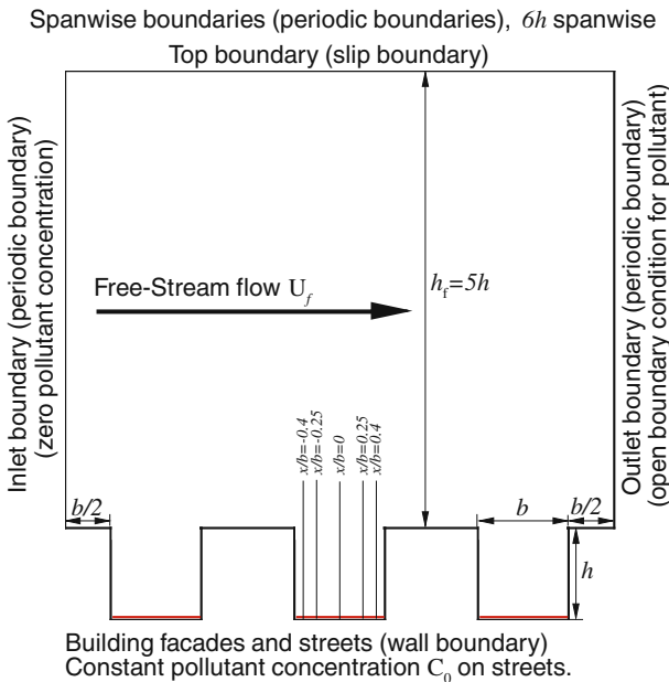
Fig. 1 Computational domain
