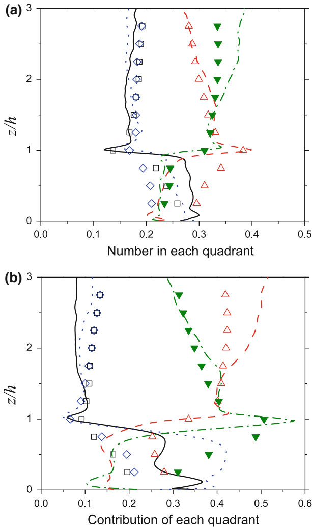
Fig. 12 Vertical profiles of a relative number and b relative contribution to (u''w'') of events in each quadrant. Current LES: Black solid line (outward interactions), red dashed line (ejection), blue dotted line (inward interaction), green dash dot line (sweeps); Coceal et al. (2007): Black square (outward interactions), red triangles up (ejections), blue diamonds (inward interaction), green filled triangle down (sweeps)
