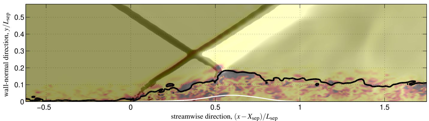
Figure 2: Snapshot from the numerical simulation: shock system (made visible by choosing a velocity-divergence-level range), pressure (black and white) and turbulent kinetic energy (color) fields (both shown on a quadratic scale for highlighting purposes), with sonic line (thick black line) and mean-separation-bubble contour (white line)
