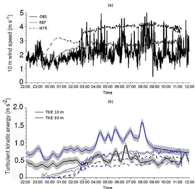
Figure 3. Observed (continuous lines) and simulated temporal evolution of 10 m wind speed (a), 10 m TKE (black line) and 30 m TKE (blue line) (b) for the REF (dotted line) and the NTR (without trees) (dashed line) simulations. Simulated fields are averaged over the horizontal area located downstream of the tree barrier (blue contour area of Fig. 1b). The grey shaded areas represent the error for the observational curves.
