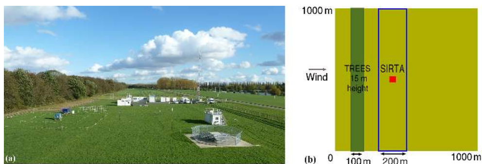
Figure 1. View of the measurement site (a) and modelling domain (b) with the tree barrier. All the simulated averaged results were taken in the blue contour area.
