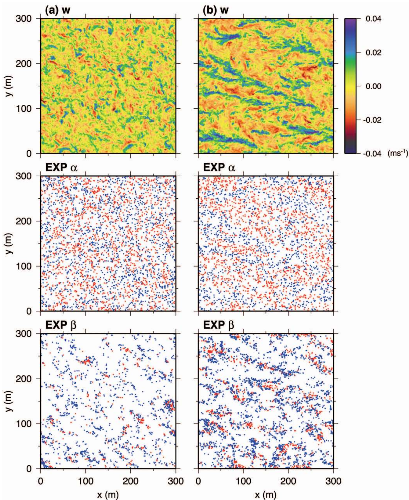
FIG. 1. (Color) Instantaneous distributions of vertical velocity (top), particles of EXP \alpha ( w_s=10^{-3} \text{ ms}^{-1} ) (middle) and of EXP \beta ( w_s=10^{-2} \text{ ms}^{-1} ) (bottom) at the horizontal cross sections ( z=10 \text{ m} ) at t^*=0.4 . Here the red and blue dots represent the particles with upward and downward vertical velocities, respectively; (a) EXP OA, (b) EXP LA.
