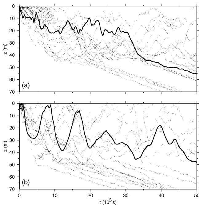
FIG. 4. Tracks of the vertical positions of particles. One typical track is shown by a thick line in each figure; (a) EXP OA_ \alpha , (b) EXP LA_ \alpha .
