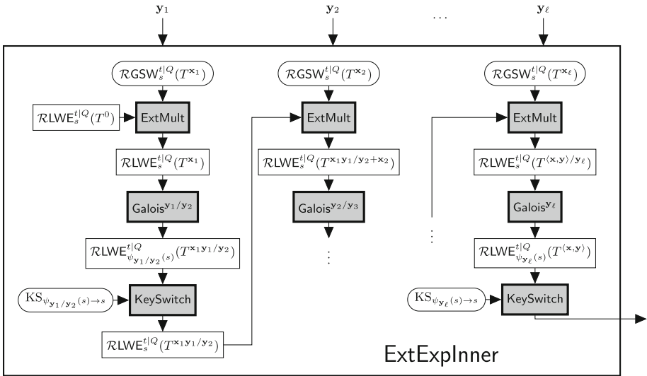
Fig. 2. Optimized ExtExplnner (external inner product in exponent) overview
