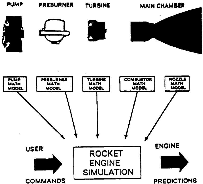
Figure 2-1. A Rocket Performance Simulation Consist of Component-By-Component Models
