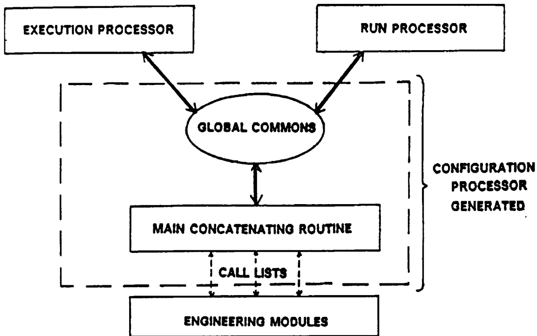
Figure 3-2. ROCETS Global Communication
