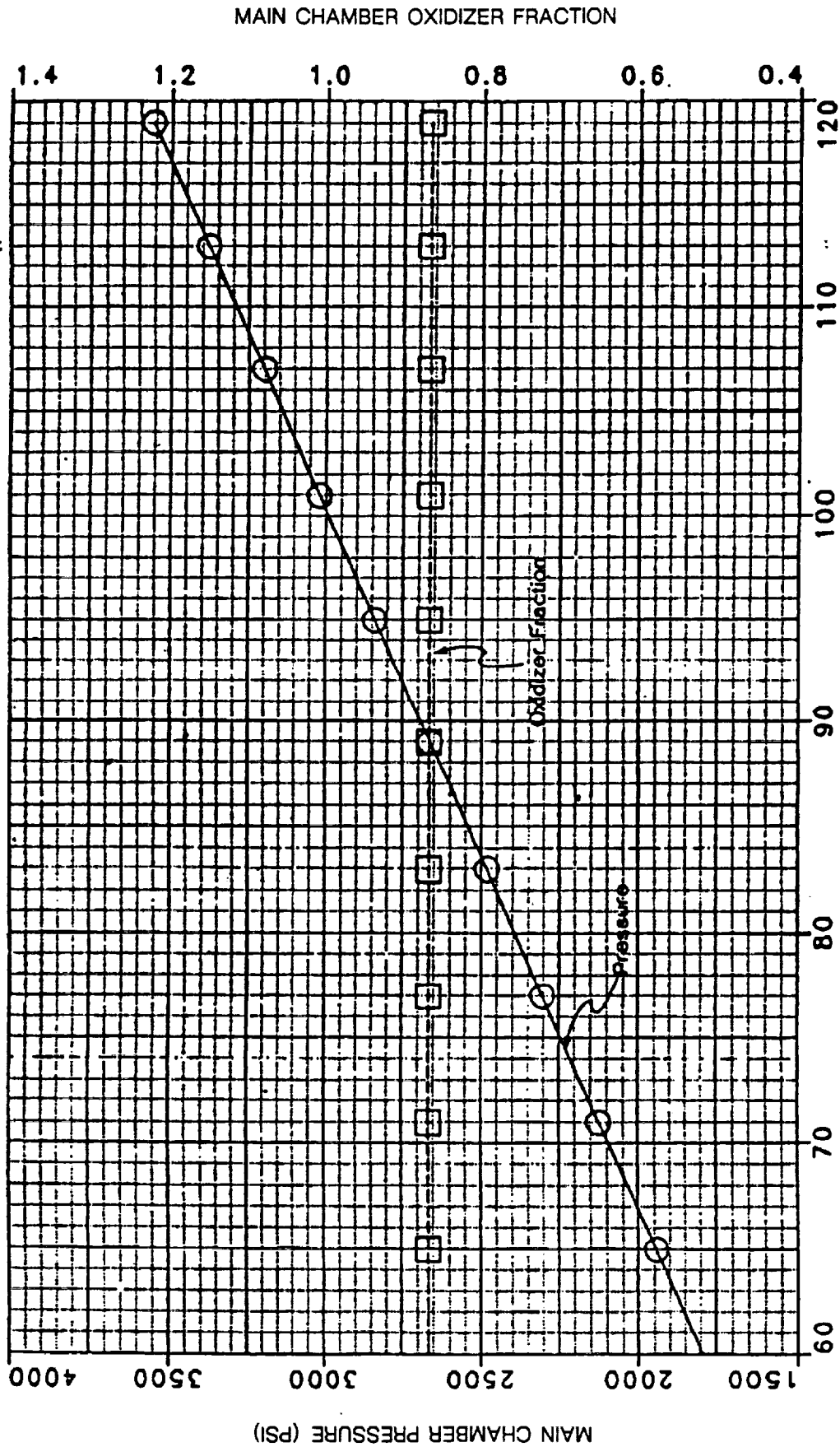
Figure 5-1 - Main Chamber Conditions as a Function of RPL
