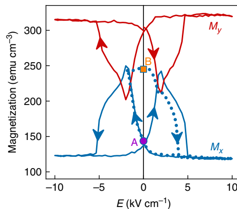
Fig. 3 Strain-mediated electrical control of macroscopic magnetization in LSMO:PMN-PT. In-plane magnetization components M_x (blue) and M_y (red) versus electric field E . Remanent states A (purple dot) and B (orange square) were achieved via the minor loop shown for M_x (dotted blue line). Data were obtained after applying and removing 1 kOe along the measurement direction, using sample A once it had undergone 30 bipolar electrical cycles (Supplementary Note 9). Similar major loops of M_x(E) were obtained for samples B and C (Supplementary Note 10). All data were obtained at room temperature. Source data are provided as a Source Data file.
