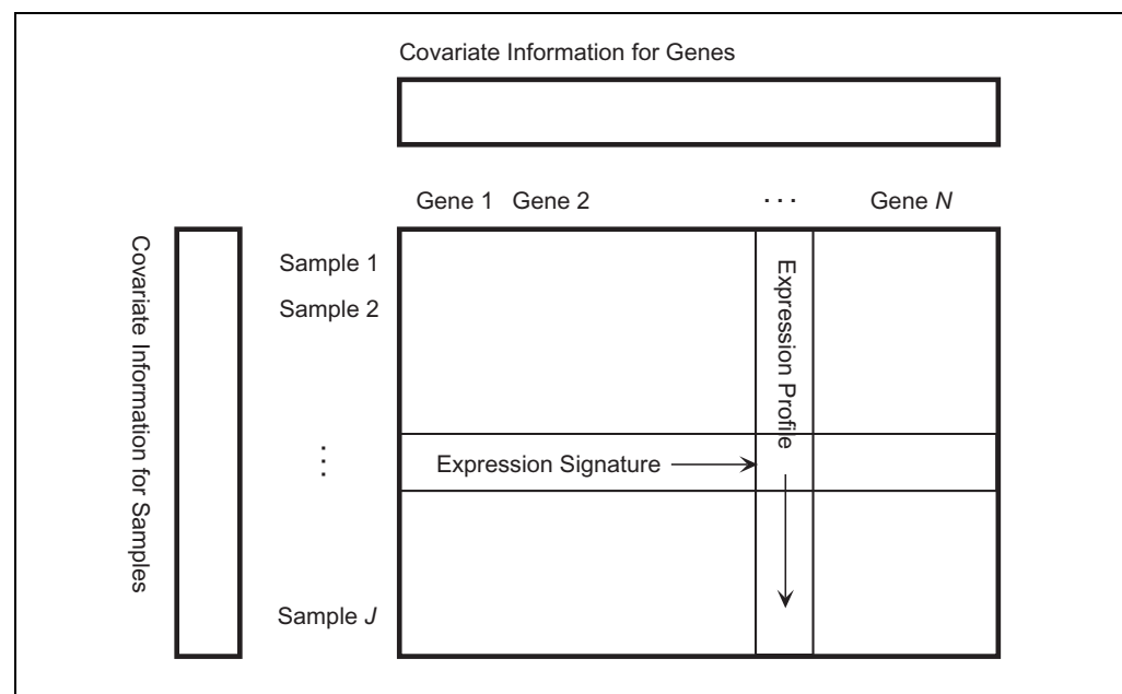
Figure 1: Schematic view of gene expression data. Expression values can be considered as a matrix where the vertical axis represents samples and the horizontal axis represents genes. Expression values for a given sample constitute an expression signature, and expression values for a given gene constitute an expression profile. Covariate information for samples and genes can be represented outside this matrix
