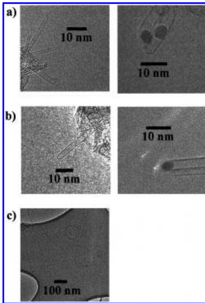
Figure 11. TEM images of SWNTs. (a) Left part: high-resolution image showing closed nanotube ends in the CVD material synthesized from the \text{Fe}/\text{Mo} /hybrid catalyst. Right part: a small fraction of SWNTs contain metal particles at their ends in the same material. (b) High-resolution TEM images of nanotubes in the materials synthesized from the \text{Fe}/\text{Ru}/\text{Al}_2\text{O}_3 catalyst. Left part: a SWNT with closed end. Right part: a SWNT with metal particle at the end. (c) Disconnected and circular tubes in the CVD material synthesized by using the \text{Fe}/\text{Ru}/\text{Al}_2\text{O}_3 catalyst.
