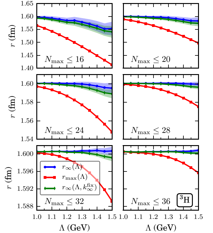
FIG. 5. Extrapolated ground-state (point-proton) radii r_\infty(\Lambda) (circles) for {}^3\text{H} with the NNLO opt NN interaction. The different panels correspond to different NCSM model space truncations from \max(N_{\text{max}}) = 16 to \max(N_{\text{max}}) = 36 . The bands estimate uncertainties from subleading IR corrections. The squares denote the maximum radius computed with the NCSM as a function of \Lambda and model space truncation.
