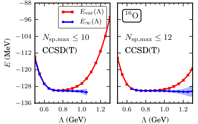
FIG. 21. Extrapolated energy E_\infty(\Lambda) (circles) for {}^{16}\text{O} . The different panels correspond to different model space truncations. The bands estimate uncertainties from subleading IR corrections. The squares denote the minimum energy computed with the Lambda-CCSD(T) as a function of \Lambda .
