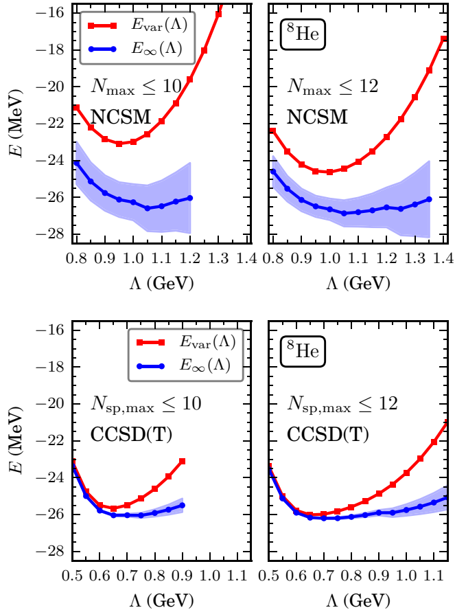
FIG. 20. Extrapolated energy E_\infty(\Lambda) (circles) for {}^8\text{He} from the NCSM (upper panels) and the coupled-cluster method (lower panels) with different model space truncations. The band estimates uncertainties from subleading IR corrections. The squares denote the minimum energy computed with the respective method as a function of \Lambda .
