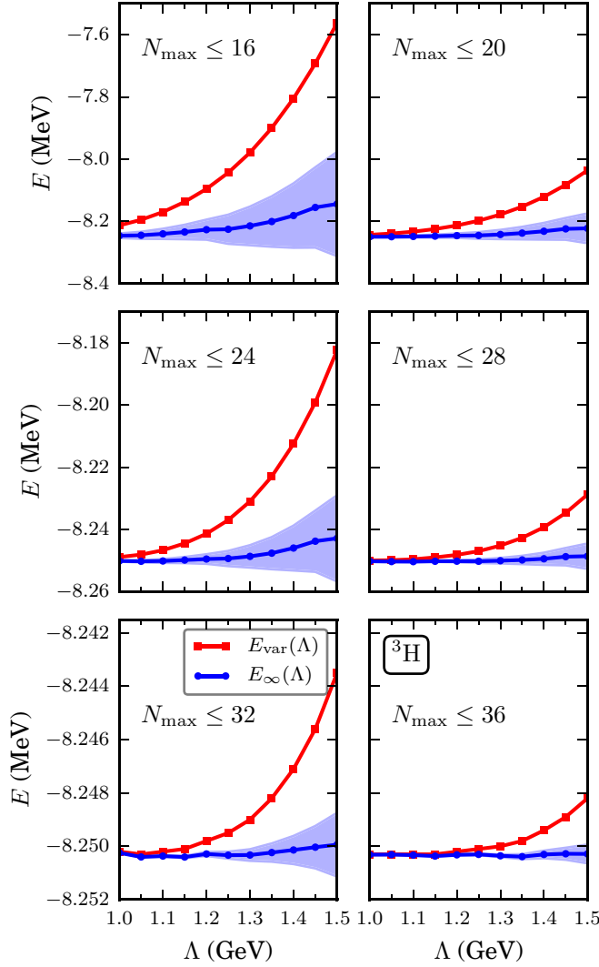
FIG. 4. Extrapolated energy E_\infty(\Lambda) (circles) for {}^3\text{H} with the NNLO opt NN interaction. The different panels correspond to different NCSM model space truncations from \max(N_{\text{max}}) = 16 to \max(N_{\text{max}}) = 36 . The bands estimate uncertainties from subleading IR corrections. The squares denote the minimum energy computed with the NCSM as a function of \Lambda .
