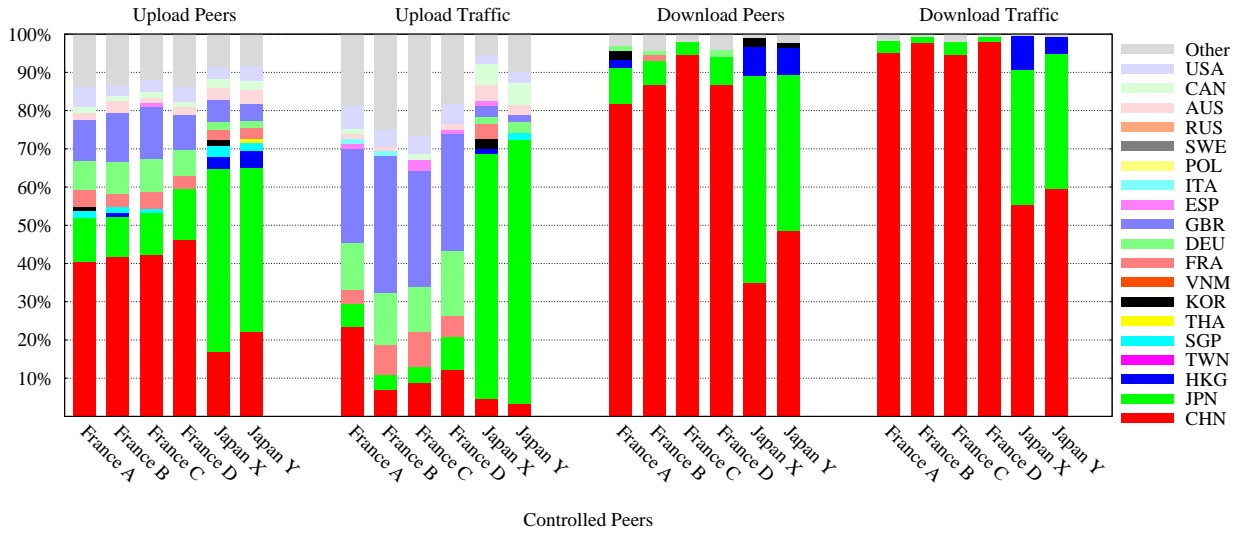
Figure 8: SOPCast: geographic location of traffic and peers (Japan-France experiment).
