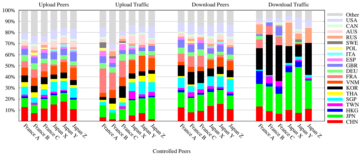
Figure 9: TVUPlayer: geographic location of traffic and peers (Japan-France experiment).
