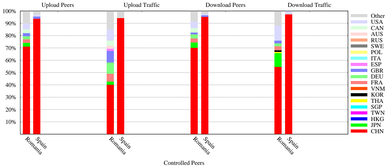
Figure 11: PPLive: geographic location of traffic and peers (Romania-Spain experiment).
