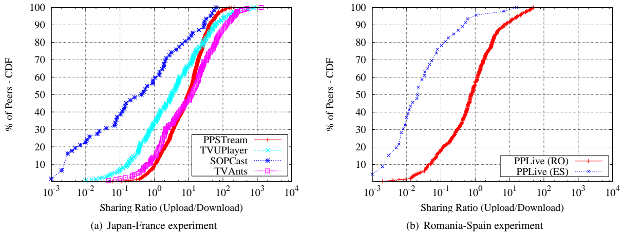
Figure 2: Traffic sharing ratio (Upload/Download). The ratio evaluates the level of collaboration between peers. When ratio is above 1, our peer is altruistic; when equal to 1, the exchange is fair; below 1 our peer take advantage of the resources of others.
