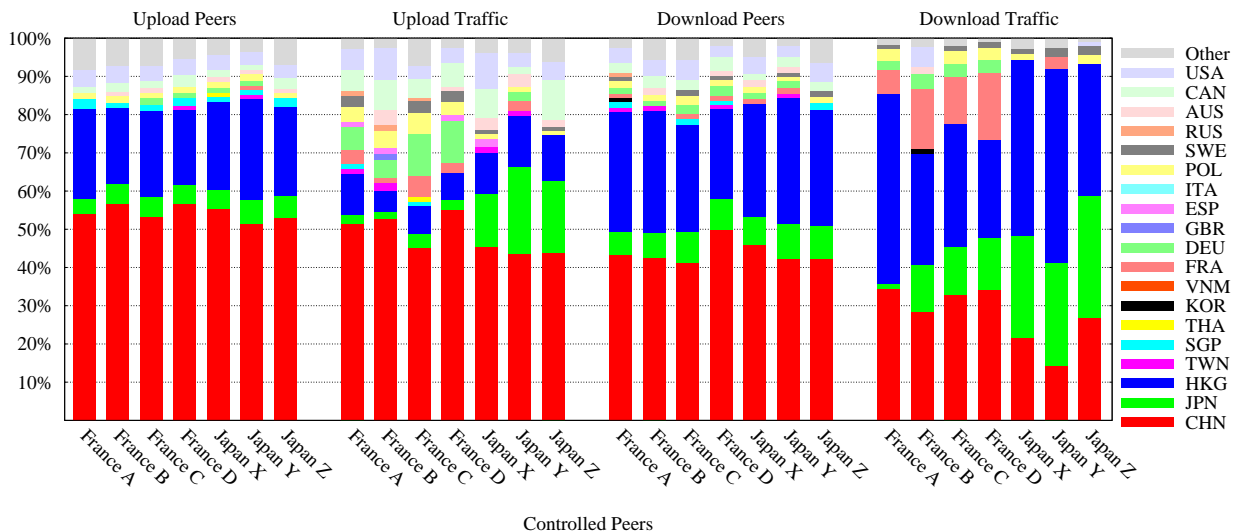
Figure 10: TVAnts: geographic location of traffic and peers (Japan-France experiment).
