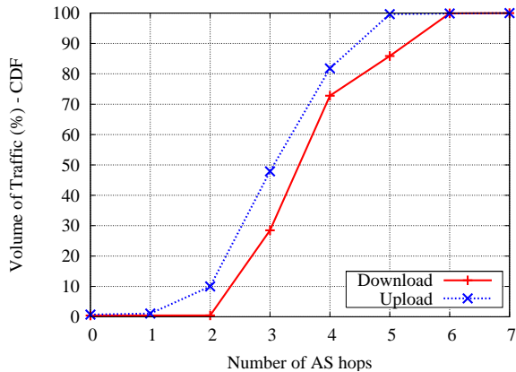
Figure 6: Distance in number of AS hops in the Japan-France experiment (Ex: SOPCast).
