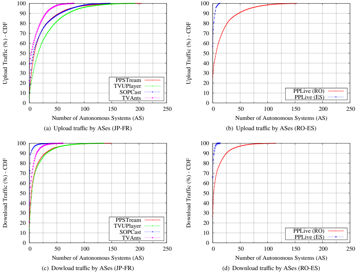
Figure 5: Traffic by Autonomous Systems (ASes). (a)-(b): Japan-France experiment; (b)-(d): Romania-Spain experiment.
