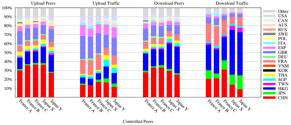
Figure 7: PPStream: geographic location of traffic and peers (Japan-France experiment).
