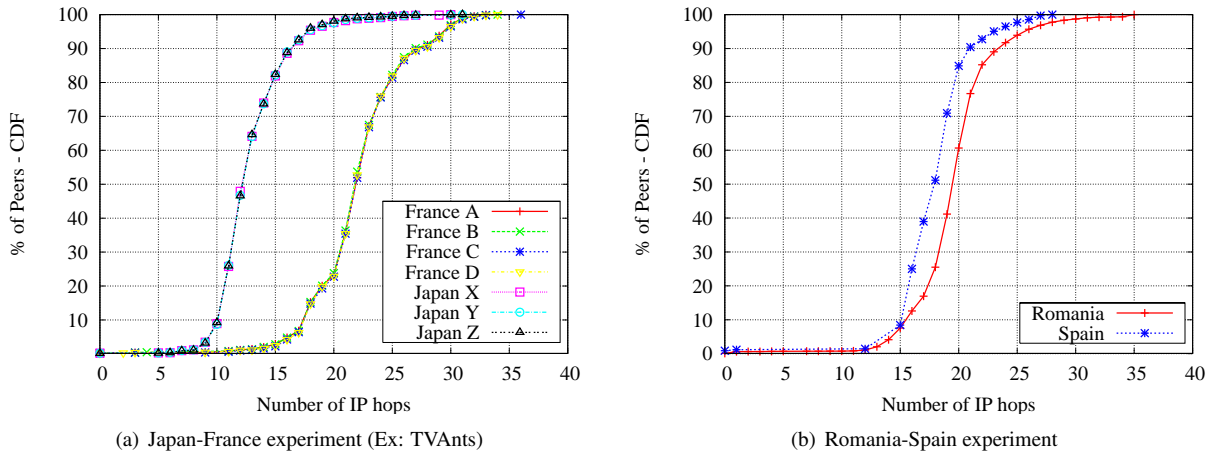
Figure 4: Distance in number of IP hops between our controlled peers and remote peers on the Internet.
