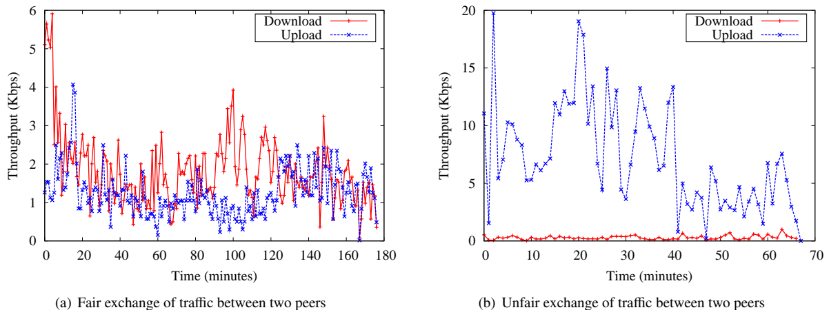
Figure 3: Examples of traffic exchange between a controlled peer and a remote peer on the Internet (Ex: PPSTream).
