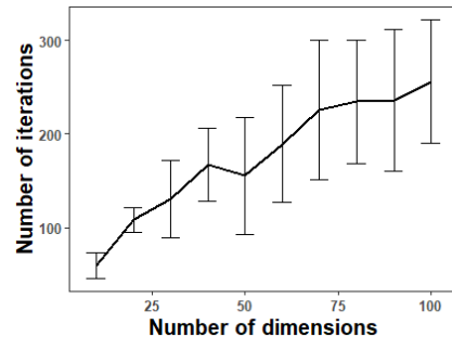
Figure 8: Number of iterations to converge
