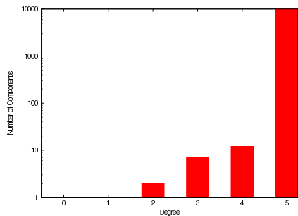
Figure 1: Degree Distribution
