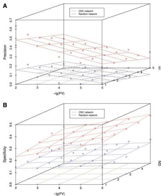
Figure 5. Hub-based functional prediction. (A) The relationship among PV, GN and precision in the CNC network. (B) The relationship among the PV, GN and specificity in the CNC network. Random networks are shown for comparison.
