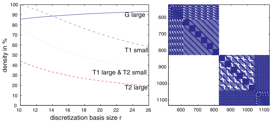
Fig. 1 Density rates of the sparse block matrices as a function of the discretization basis size r (left), and sparsity structure for the two largest block matrices of the T2 condition for r = 12 (right)
