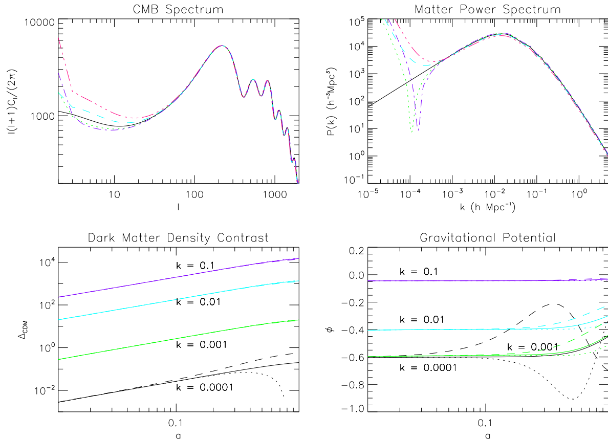
FIG. 3. (Colour online) The power spectra for the large-scale structure of the f(T) gravity model with f(T) = T - \mu^{2(1+n)} / (-T)^n . Upper-left Panel: the CMB spectrum for different values of n – 0 (black solid curve), 0.1 (green dotted curve), -0.1 (cyan dashed curve), 0.2 (purple dash-dotted curve) and -0.2 (pink dash-triple-dotted curve). Upper-right Panel: the same as the upper-left panel, but for the matter power spectrum at redshift 0 (today). Lower-left Panel: the late-time evolution of the dark matter density contrast \Delta_{\text{CDM}} on different scales (as indicated besides the curves); three values of n have been considered – n = 0.0 (solid curves), 0.1 (dotted curves) and -0.1 (dashed curves). Lower-right Panel: the same as the lower-left panel, but for the late-time evolution of the gravitational potential \phi on different scales. The physical parameters are the same as listed in the caption of Fig. 1, and three species of massless neutrinos are used.
