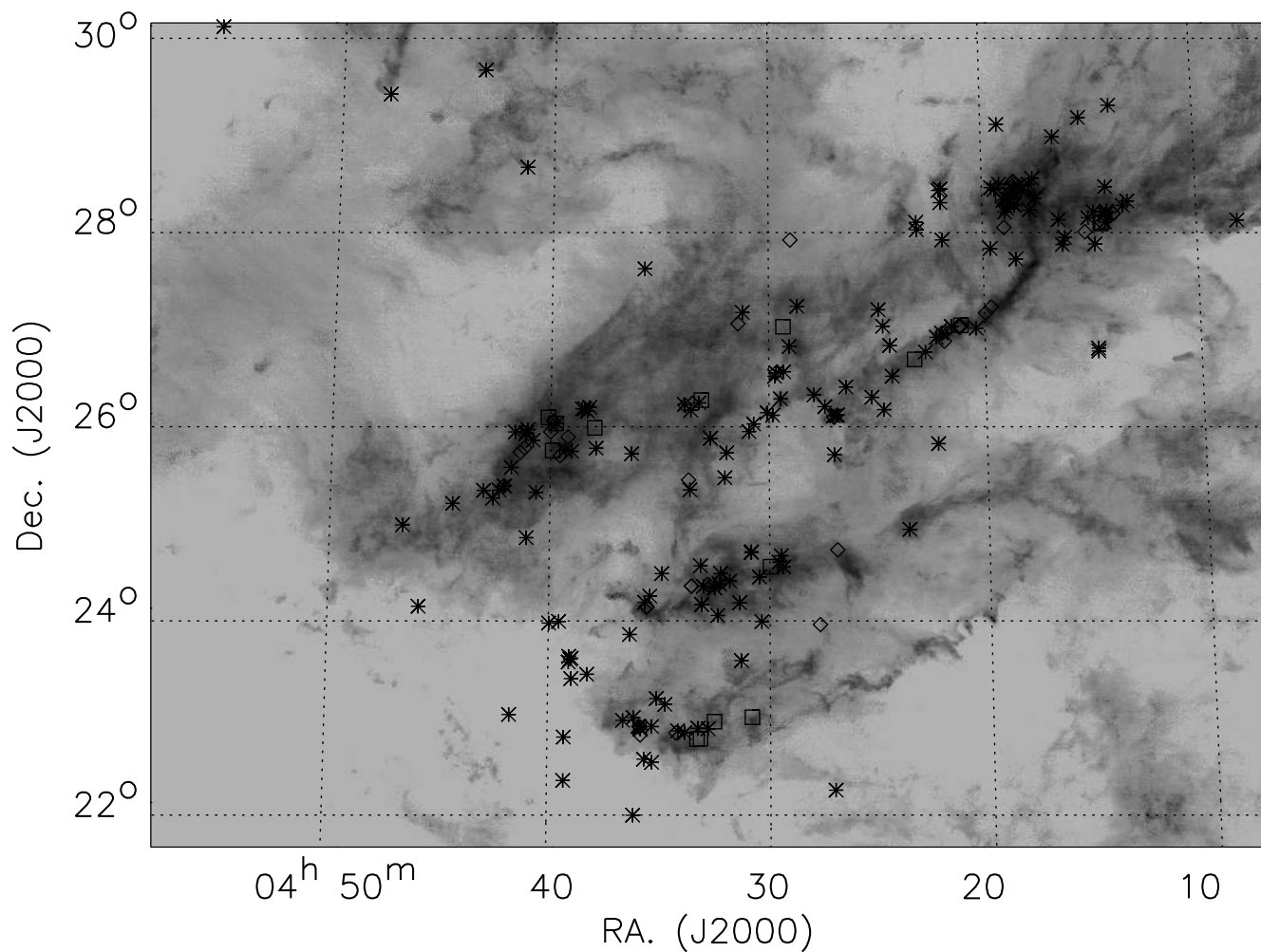
Fig. 14.— Locations of young stars in Taurus superimposed on map of the H_2 column density. The stellar positions are from Kenyon (2007). The diamonds indicate diffuse or extended sources (of which there are 44 in the region mapped), the squares indicate Class I or younger stars (18), and the asterisks indicate T-Tauri stars (168). It is evident that the diffuse and younger sources are almost without exception coincident with regions of relatively large column density, while the older stars show a much larger probability of being found in regions of lower column density.
