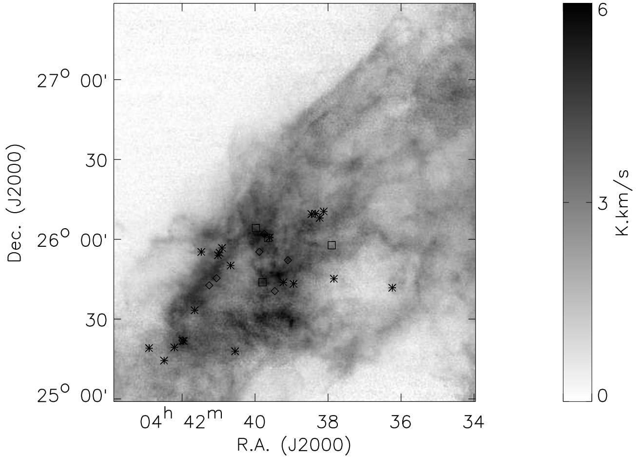
Fig. 19.— ^{13}\text{CO} integrated intensity image showing the molecular ring in Heiles’ Cloud 2 centered at 4^{\text{h}}40^{\text{m}}30^{\text{s}} + 25^{\circ}45' . We also see the very well-defined planar boundary centered at 4^{\text{h}}38^{\text{m}}30^{\text{s}} + 26^{\circ}50' . The ^{12}\text{CO} boundary in this region is not at all sharp, having a hair-like appearance as seen most clearly in Figure 13. The diamonds indicate diffuse or extended young stellar sources, the squares indicate Class I or younger stars, and the asterisks indicate T-Tauri stars.
