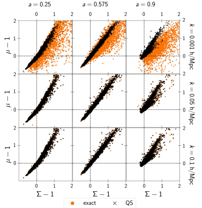
FIG. 4. Same as in Figs. 2 and 3, but for the full class of Horndeski models with the restriction of the speed of gravitational waves imposed only at z = 0 .
