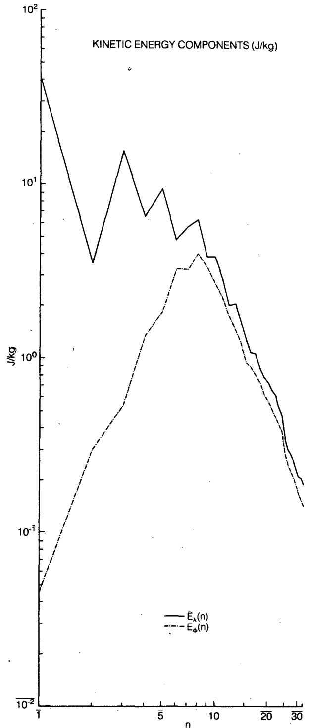
FIG. 7. Integrated zonal and meridional kinetic energy spectra for January.
