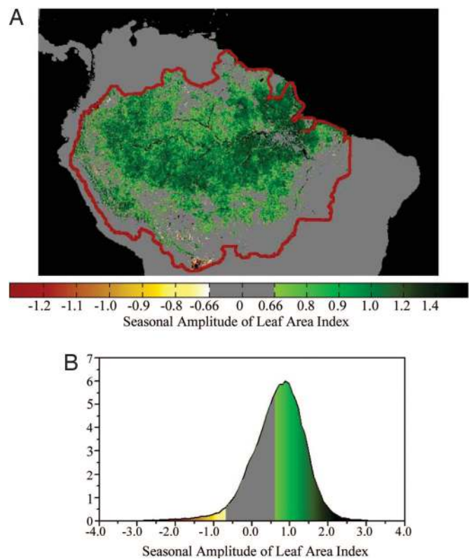
Fig. 2. Seasonal amplitude of LAI. (A) Color-coded map of LAI amplitudes greater than 0.66 or less than -0.66 ; this threshold (0.66) is the smallest LAI difference discernable with the MODIS LAI data set (see SI Materials and Methods). In regions with dry seasons longer than 3 months, the amplitude is calculated as the difference between the maximum 4-month average LAI in the dry season minus the minimum 4-month average LAI in the wet season. Where the dry season is three or fewer months, the amplitude is calculated as the difference between the dry-season average LAI and the minimum 4-month average LAI in the wet season. The dry and wet seasons are defined based on the precipitation data set at 15' spatial resolution (see SI Materials and Methods). Thus, the seasons vary spatially and interannually. (B) Distribution of LAI amplitude for all Amazon rainforest pixels. The color scheme is similar to that in A.
