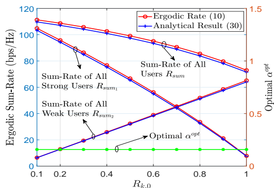
Fig. 3: Achievable ergodic sum-rate and optimal \alpha^{\text{opt}} vs R_{k,0} .
