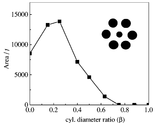
FIG. 6. Area, normalized to the filling fraction f , of the first attenuation-band-overlap observed in transmission spectra taken along the \Gamma J and \Gamma X directions, in the reduced-symmetry honeycomb lattice. The line is a guide for the eye.
