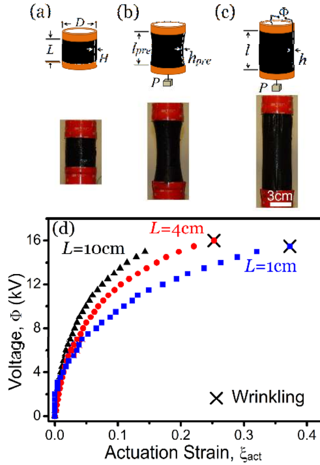
FIG. 1. Response of cylindrical actuators made of elastomer sheets without fibers. (a) In the reference state, the elastomer is undeformed. (The elastomer is black because of the carbon electrode coating). (b) The cylinder is in a pre-stretched state due to an applied force P . Note the formation of a waist in the central region of the actuator. (c) In the actuated state, the membrane is subject to both the force P and voltage \Phi . The red ends are stiff rings on which the elastomer is attached. The three states are illustrated with both schematics and photographs of a cylinder of length L = 4 cm. Cylinders of length L = 1 cm and 4 cm formed wrinkles before electric breakdown. (d) For cylinders of different lengths, the actuation strains were recorded as the voltage was ramped up. The successive data points were recorded at equal time intervals of 10s. Each run of the experiment was terminated at electric breakdown.
