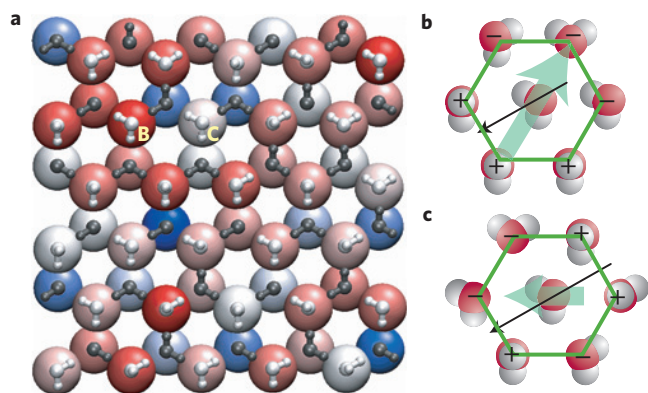
Figure 5 | Spatial variation of dipole magnitude. a , A top view of the spatial distribution of dipole moments for the (0001) surface of ice Ih (equivalent to layer 1 and 2 in Fig. 1). The image is a composite, where the magnitude of the water dipole is represented by a coloured sphere; red indicates a low dipole, white an intermediate dipole, and blue a large dipole. The ball-and-stick water molecules are superimposed on the spheres, where layer 1 molecules are in white and layer 2 molecules are in grey. b,c Two specific examples taken from the points marked B and C in a , respectively, indicate how local electric fields (denoted by light green arrows) created by the net effective charges on the dangling protons (+ve) and dangling lone pairs (–ve) can either reduce ( b ) or enhance ( c ) the dipole moments (indicated by black arrows) of molecules in the top layer. Note that the layer 2 molecules have been hidden in b and c to emphasize the surface geometry.
