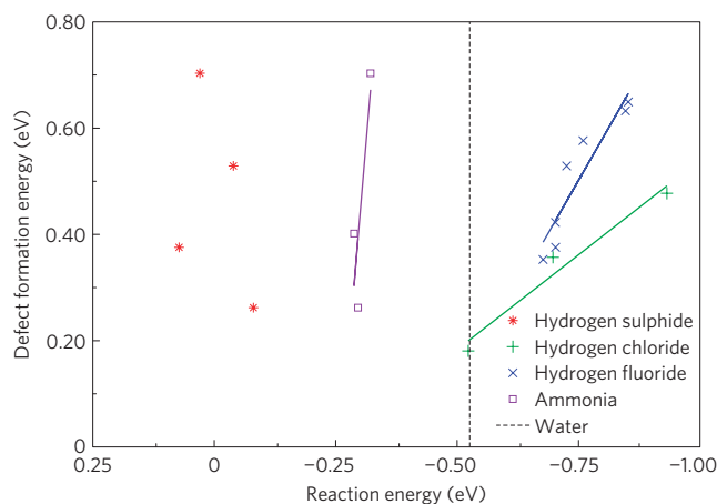
Figure 6 | Reactivity of various gases at surface vacancies. The figure shows the substitution reaction energy for HF, HCl, \text{H}_2\text{S} and \text{NH}_3 with water molecules at the (0001) surface of ice. The vacancy formation energy reflects how strongly the water molecule is bound. The reaction energy corresponds to the energy released on displacement of a water molecule at the surface to an atop location. The dashed line signifies the attack of a gaseous water molecule at a surface site and displacement of a water to an atop location. Right of the dashed line indicates displacement of surface bound water in a competitive reaction between a gas molecule and gaseous water. Negative reaction energies indicate displacement of surface bound water when the partial pressure of gaseous water is low.
