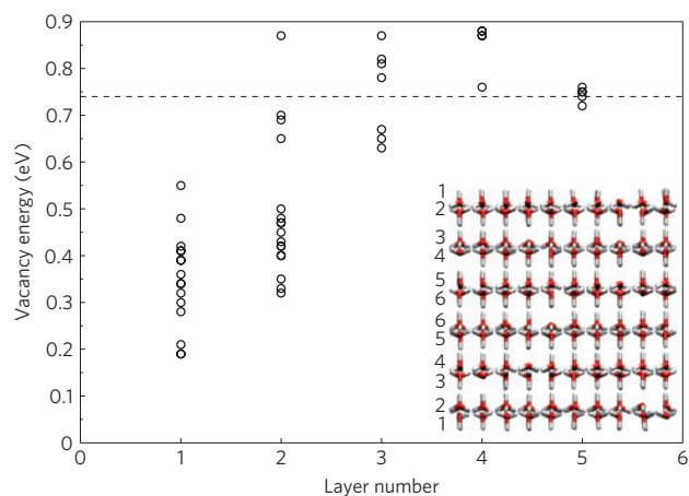
Figure 2 | Distribution of vacancy formation energies in an ice slab. Vacancy formation energies computed for a 6-bilayer slab of (0001) ice Ih (containing 12 layers in total). The inset figure corresponds to the configuration in Fig. 1, but viewed along the [010] axis, that is, in cross-section. Layer 1 is the external layer containing undercoordinated water molecules. Layer 2 molecules notionally have four hydrogen bonds per water. The vacancy energy generally increases as a function of the depth into the crystal. The dashed line indicates the vacancy formation energy ( 0.74 \text{ eV} ) for the crystal bulk. Note that the variance in vacancy energy in the bulk is 0.025 \text{ eV} , and hence the dashed-line width overemphasizes the variance.
