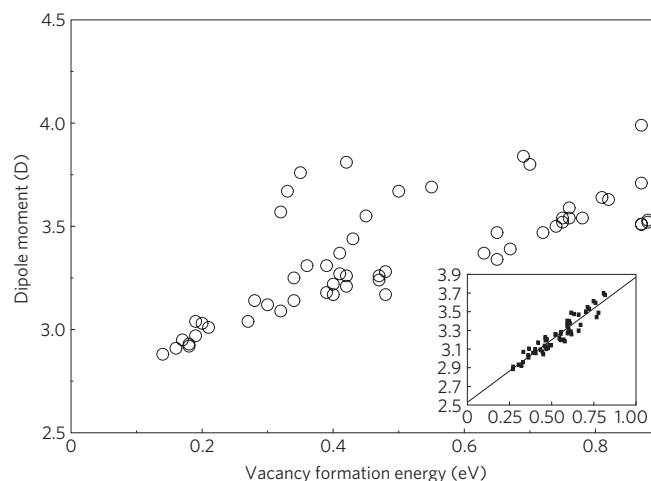
Figure 4 | Correlation between vacancy formation energies and dipole moments. Scatter plot of the dipole moments and associated vacancy formation energies calculated for over 50 unique sites within a 6-bilayer Ih slab that exposes (0001) surfaces, showing a general positive correlation between dipole moment and vacancy formation energy. The inset is a plot of the unrelaxed defect formation energy versus dipole moment with same axis labels as the main figure.
