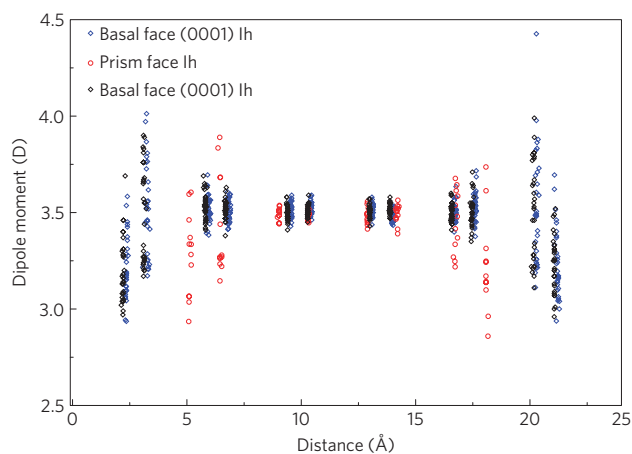
Figure 3 | Dipole-moment distribution in ice slabs. The dipole moment of individual molecules within two 6-bilayer slabs of ice Ih exposing the (0001) surface, and within a 4-bilayer slab exhibiting the prismatic face. The two different samples for the basal face correspond to slabs with different degrees of proton disorder at the surface. In the interior of the crystal slab, the dipole moment is approximately 3.5 Debye, but for all the structures considered here the dipole moments vary greatly towards, and at, the crystal surface.
