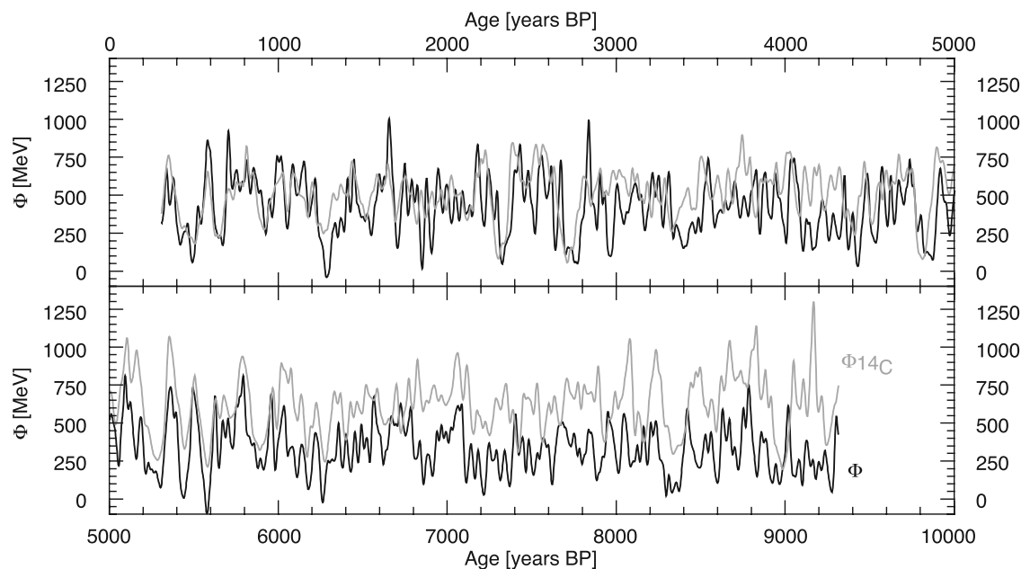
Figure 7. Comparison of \Phi reconstructed from ^{10}\text{Be} (black curve) with \Phi reconstructed from the ^{14}\text{C} production rate ( \Phi_{14\text{C}} , gray curve). Both \Phi records are high pass filtered (cutoff frequency 1/2000 \text{ years}^{-1} ) to remove their different long-term trends.
