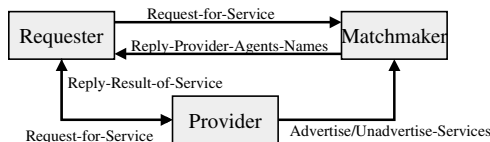
Figure 1. Service brokering vs. matchmaking.
