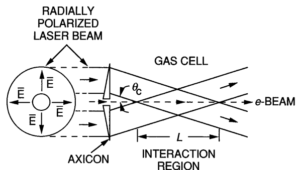
FIG. 1. Inverse Cherenkov acceleration configuration [3]. A radially polarized laser beam is focused by an axicon onto the e beam at the Cherenkov angle \theta_C inside a gas-filled region, resulting in energy exchange occurring over an interaction length L .
