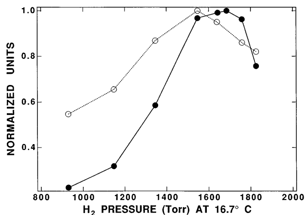
FIG. 5. Gas pressure dependence results. The solid curve is the model prediction, where the normalized maximum electron acceleration is plotted as a function of pressure. The dashed curve is the data, where the normalized width of the measured central subspectrum is plotted as a function of pressure.
