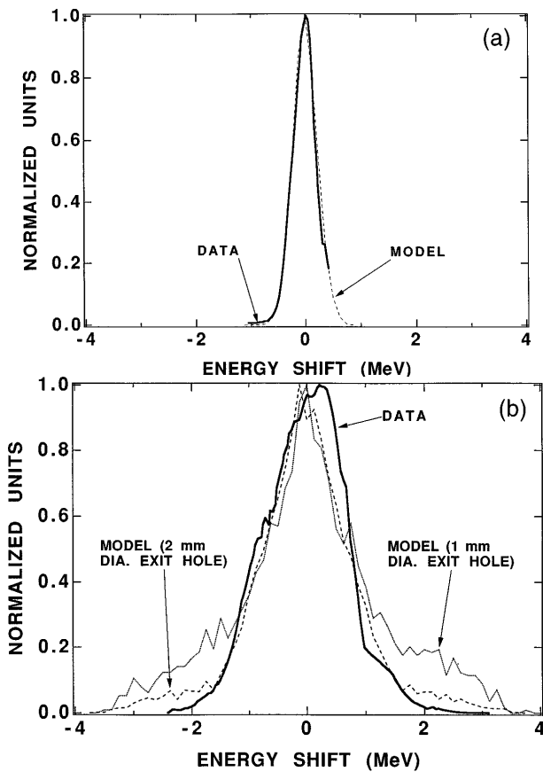
FIG. 3. Electron-beam energy spectra. Solid curves are the subspectra data that have been spliced together (see text), dashed and dotted curves are the model predictions [8]. (a) With no laser present and after traveling through the gas cell filled with 2.2 atm H 2 at 16.7 °C. (b) With 580 MW of laser peak power delivered to the interaction region and measured at constant spectrometer detector gain.
