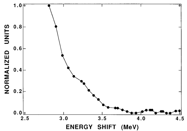
FIG. 4. Electron-beam energy subspectrum (single shot data) of the high energy region obtained with the spectrometer detector set to maximum gain. All the other conditions are the same as in Fig. 3.
