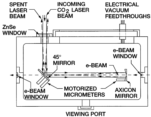
FIG. 2. Schematic plan view of the gas cell where the inverse Cherenkov interaction occurs. Note that an axicon mirror is used rather than an axicon lens, as shown in Fig. 1. The optics in the gas cell can be adjusted remotely.
