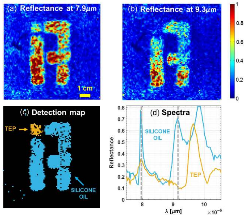
Fig. 6 Composite hypercube that depicts the IARPA logo drawn onto HDPE using two different chemicals: (a) reflectance image at 7.9 μm, (b) reflectance image at 9.3 μm, (c) detection map indicating the two different chemicals, and (d) reflection spectra for the two different chemicals. Video 2 shows sample preparation, acquisition, and the resulting hypercube (Video 2, 13.3 MB, MP4 [URL: https://doi.org/10.1117/1.OE.59.9.092003.2 ]).
