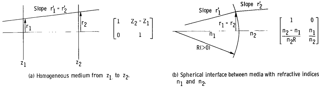
Figure 14. - Ray paths and corresponding ABCD matrices.
