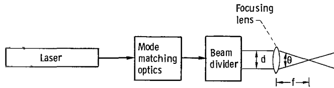
Figure 12. - General dual scatter transmitting optical system.
