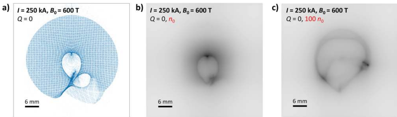
FIG. 3. Synthetic 13 MeV proton-deflectograms assuming I = 250 \text{ kA} , B_0 = 600 \text{ T} , and Q = 0 . Panel (a) shows the results of test-particle calculations, while panels (b) and (c) display the results of self-consistent PIC simulations run with different input plasma densities: (b) n_0 \sim 10^{18} \text{ cm}^{-3} at the left side of the simulation box (matching the experimental data) and (c) 100 \times n_0 \sim 10^{20} \text{ cm}^{-3} . The black horizontal bars give the spatial scale at the RCF detection plane.
