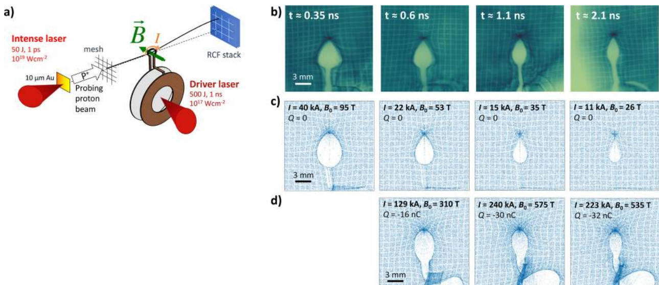
FIG. 2. (a) Sketch of the proton-deflectometry setup (not to scale). (b) Zoomed RCF data for 13 \pm 1 MeV protons from shots with varying delay between the lasers, \Delta t = 0.25, 0.5, 1, and 2 ns (from left to right). The labels give the probing times, accounting for the protons' time-of-flight between the foil and the coil. (c) Corresponding synthetic proton-deflectograms, obtained from numerical simulations of the proton trajectories through 3D B-field maps matching the experimental data (labelled by the discharge current I and the corresponding strength of the B-field at the coil center B_0 ). (d) Idem setting the B-field strength to the average value inferred from the B-dot data at the corresponding times [orange diamonds in Fig. 1(b)] and adding a charge of magnetized plasma electrons Q , which allows matching the synthetic and experimental widths of the void-bulb. The white/black horizontal bars give the spatial scale at the RCF detection plane, corresponding to a magnification of 10 with respect to the plane of the coil axis.
