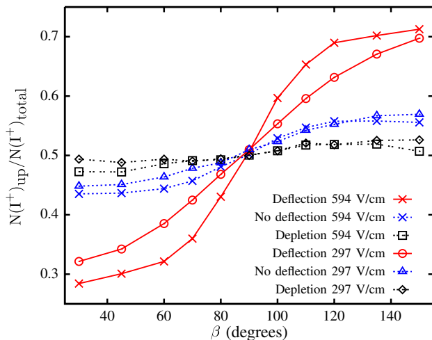
FIG. 4 (color online). Orientation, represented by N(I^+)_{\text{up}}/N(I^+)_{\text{total}} , as a function of \beta ; see text for details.
