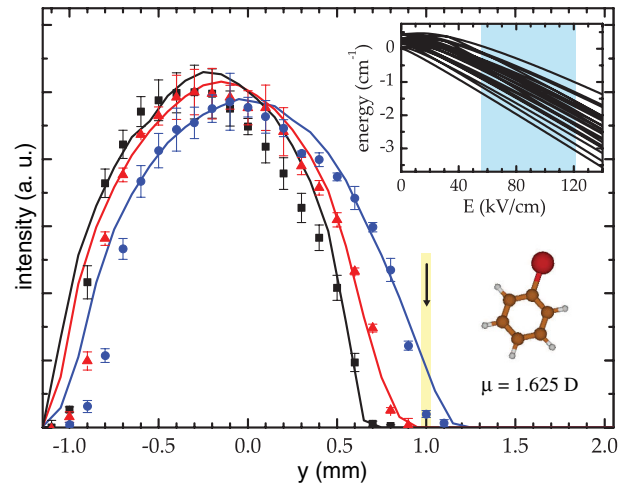
FIG. 2 (color online). The vertical profile of the molecular beam measured by recording the laser-induced \text{I}^+ signal (see text). The experimental data are shown by (black) squares (deflector off), (red) triangles (5 kV), and (blue) circles (10 kV), together with the corresponding simulated profiles. In the inset the energies of the lowest quantum states of iodobenzene are shown as a function of the electric field strength. The shaded area represents the range of field strengths present in the detector for a voltage of 10 kV. The value of the dipole moment of iodobenzene [22] is given below the molecular model.
