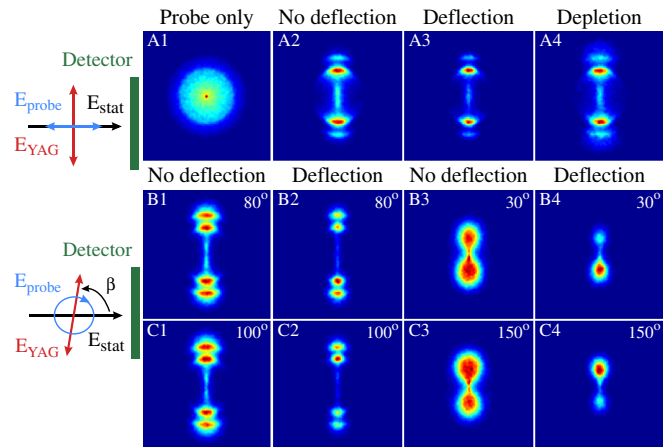
FIG. 3 (color online). I^+ ion images, recorded when the probe pulse Coulomb explodes the iodobenzene molecules, illustrating alignment and orientation. The polarization state of the YAG and the probe pulse with respect to the detector plane and the static field is shown schematically at the left. Images labeled “no deflection” are recorded at lens position y = 0.0 mm, “deflection” at y = 1.0 mm, and “depletion” at y = -0.9 mm, the latter two with the deflector at 10 kV (see Fig. 2). The value of \beta is shown for each image in row B and C. The intensity of the YAG pulse is 8 \times 10^{11} W/cm 2 and 5 \times 10^{14} W/cm 2 for the probe pulse. E_{stat} = 595 V/cm.
