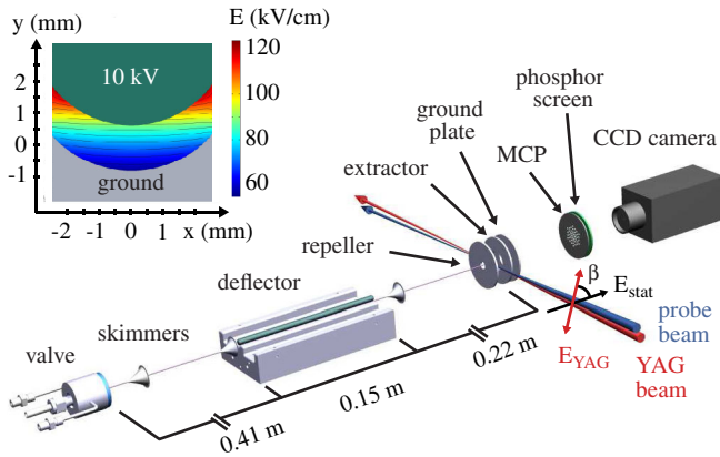
FIG. 1 (color online). Scheme of the experimental setup. In the inset, a cut through the deflector is shown, and a contour plot of the electric field strength is given.
