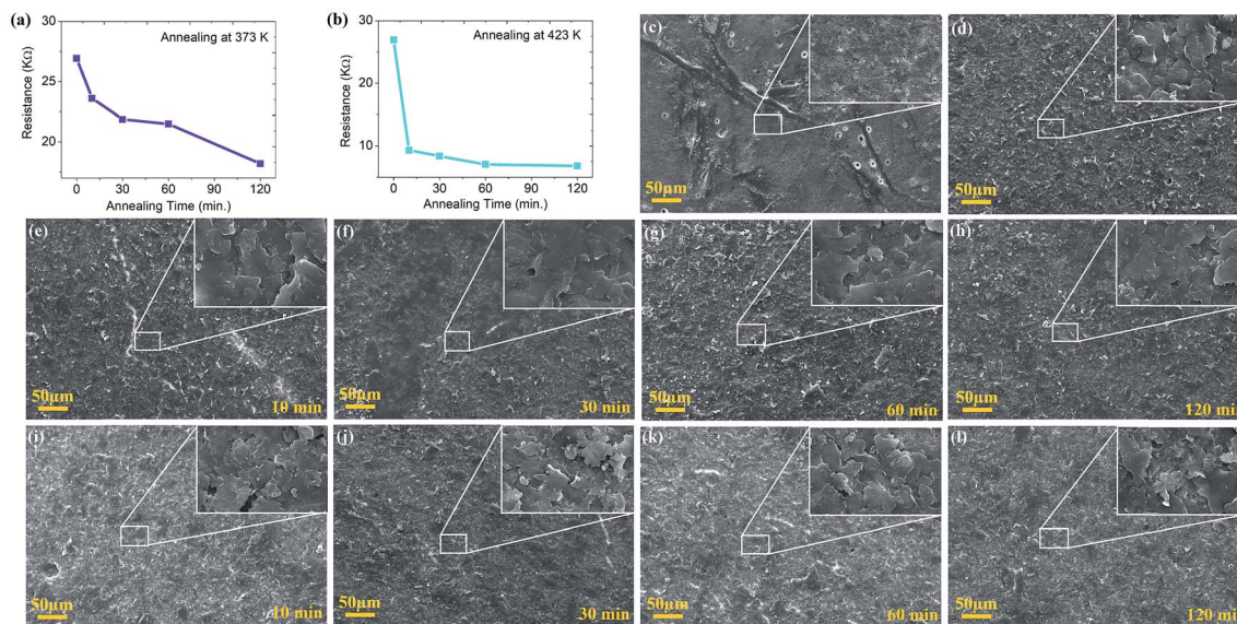
Fig. 2 Change in resistance of the device w.r.t. annealing time at annealing temperature (a) 373 K and (b) 423 K. SEM images at 500× magnification (in inset at 10× magnification) of (c) paper substrate, (d) graphene ink coated on paper substrate without annealing, (e–h) device surface after annealing at 373 K and (i–l) 423 K for 10, 30, 60, 120 min, respectively.
