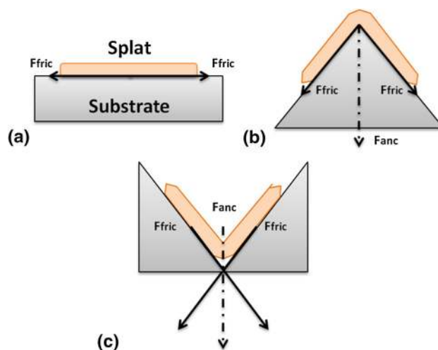
Fig. 4 Sketch of the anchoring force ( F_{Anc} ) of a splat as a function of the in-contact surface shape
