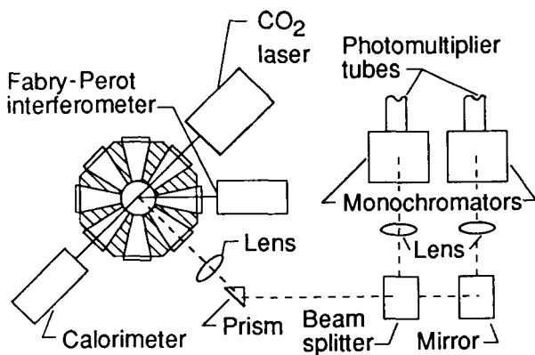
Figure 5. Laser-heated plasma.
