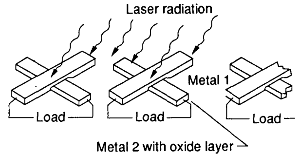
(a) Optical rectification.
