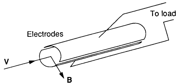
Figure 10. Simple MHD generator used in experiments.
