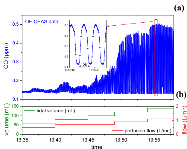
Fig. 4 a CO measurements performed by OF-CEAS on an ex vivo pig lung during slow warming after cold ischemia. The response time allows to monitor both inspiration and expiration phases imposed by the ventilator (respiratory rate is 12 per min). The baseline corresponds to CO concentration in the medical gas supply. b Lungs were progressively ventilated and rewarmed by a perfusion solution
