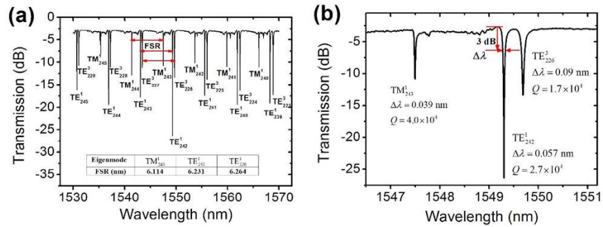
Figure 4. Transmission spectrum of the microfiber in presence of the MFIMOF microresonator with a diameter of 86.4 \mu\text{m} . (a) Mode orders corresponding to different resonance dips. The FSRs for \text{TM}_m^1 , \text{TE}_m^1 and \text{TE}_m^3 modes are also calculated (b) Enlarged transmission spectrum around 1550 nm. The FWHM and Q factors for \text{TM}_{243}^1 , \text{TE}_{242}^1 and \text{TE}_{226}^3 modes are also calculated.
