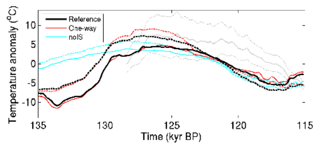
Figure 6. Comparison of modelled north-eastern Greenland annual mean (solid) and summer (June–July–August, dashed) surface temperature evolution ( 72\text{--}83^{\circ} N and 306^{\circ}33'\text{--}317^{\circ}48' E) with reconstructed temperature changes (grey) at deep ice core site NEEM ( 77^{\circ}27' N, 308^{\circ}56' E). The solid grey line is the central estimate and grey dashed lines give the estimated error range for NEEM (NEEM community members, 2013).
