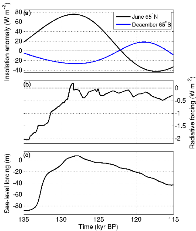
Figure 2. Prescribed model forcing. (a) Average monthly insolation anomaly at 65° N in June (black) and 65° S in December (blue) to illustrate the spatially and temporally resolved forcing (Berger, 1978), (b) combined radiative forcing anomaly of prescribed greenhouse gas concentrations relative to the present day, and (c) sea-level forcing for the ice sheet components derived from a Red Sea sea-level record (Grant et al., 2012).
