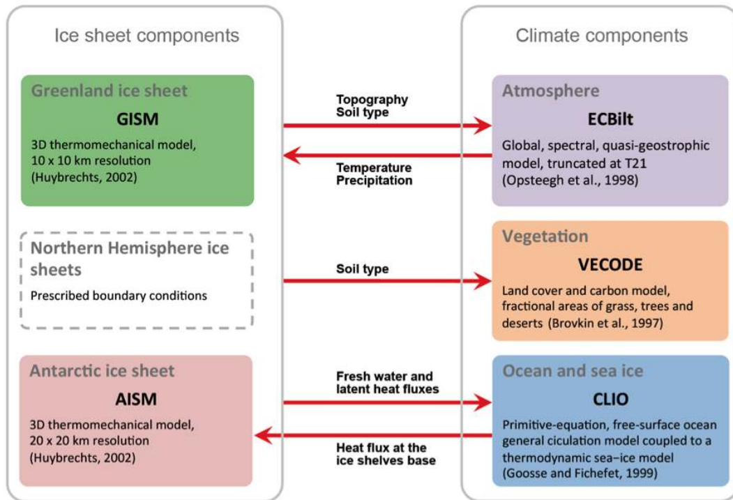
Figure 1. LOVECLIM model setup for the present study including dynamic components for the Greenland and Antarctic ice sheets and prescribed Northern Hemisphere ice sheet boundary conditions.
