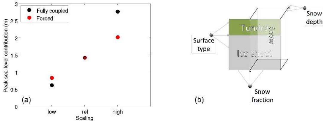
Figure 7. Scaling of sea-level contribution from the Greenland ice sheet as a function of temperature changes for the full model (black) and forced model (red) in comparison (a). Schematic of the albedo parameterisation in the land model for (partially) ice-covered areas (b), which is a function of the underlying surface type, snow fraction, and snow depth. See main text for details.
