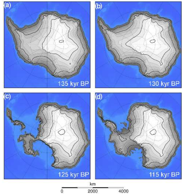
Figure 9. Antarctic grounded ice sheet geometry at 135 kyr BP (a), 130 kyr BP (b), for the minimum ice sheet volume at 125 kyr BP with a sea-level contribution of 4.4 m (c), and at the end of the reference experiment at 115 kyr BP (d).
