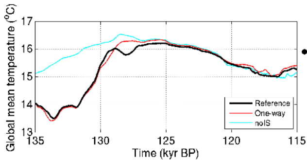
Figure 3. Global annual mean near-surface air temperature evolution of the reference run (black) compared to experiments with prescribed Greenland and Antarctic ice sheet evolution from stand-alone experiments (One-way, red) and no ice sheet changes at all (noIS, light blue). The filled circle on the right axis indicates the temperature for a pre-industrial control experiment of the reference model with present-day ice sheet configuration.
