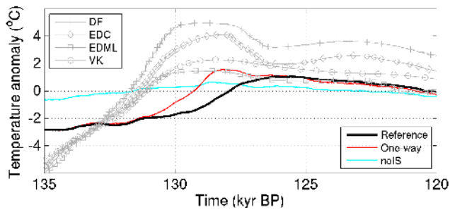
Figure 10. Comparison of modelled East Antarctic temperature evolution with reconstructed temperature changes at deep ice core sites. Modelled temperature anomalies are averaged over a region 72–90° S and 0–150° E. Ice core temperature reconstructions for the sites EPICA Dronning Maud Land (EDML; 75°00′ S, 00°04′ E), Dome Fuji (DF; 77°19′ S, 39°40′ E), Vostok (VK; 78°28′ S, 106°48′ E), and EPICA Dome C (EDC; 75°06′ S, 123°21′ E) are from Masson-Delmotte et al. (2011).
