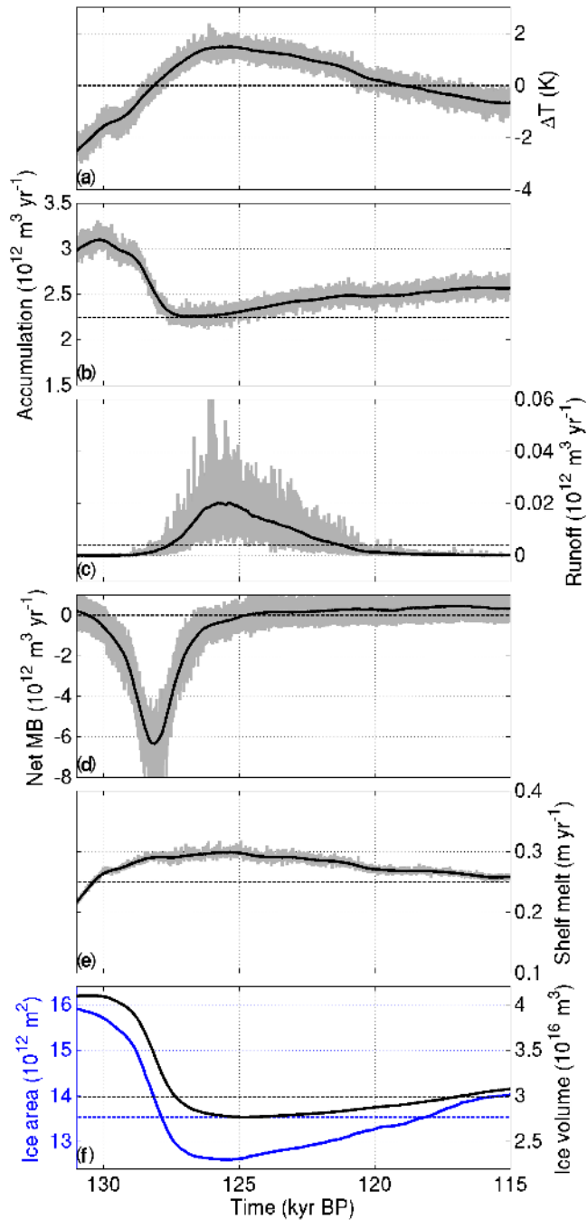
Figure 8. Antarctic ice sheet forcing and characteristics. Temperature anomaly relative to the pre-industrial period (a), accumulation (b), surface meltwater runoff (c) and net mass balance of the grounded ice sheet (d), and average sub-shelf melt rate diagnosed for the area of the present-day observed ice shelves (e). Mass balance terms (b–e) are given in water equivalent. (f) Grounded ice sheet area (blue) and volume (black). Grey lines give full annual time resolution, while black lines (and blue in f) are smoothed with a 400-year running mean. Horizontal dashed lines give the pre-industrial reference values, except for (d), where it is the zero line.
