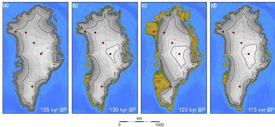
Figure 5. Greenland ice sheet geometry at 135 kyr BP (a), at 130 kyr BP (b), for the minimum ice sheet volume at 123 kyr BP with a sea-level contribution of 1.4 m (c), and at the end of the reference experiment at 115 kyr BP (d). The red dots indicate the deep ice core locations (from south to north-west: Dye-3, GRIP, NGRIP, NEEM, Camp Century).
