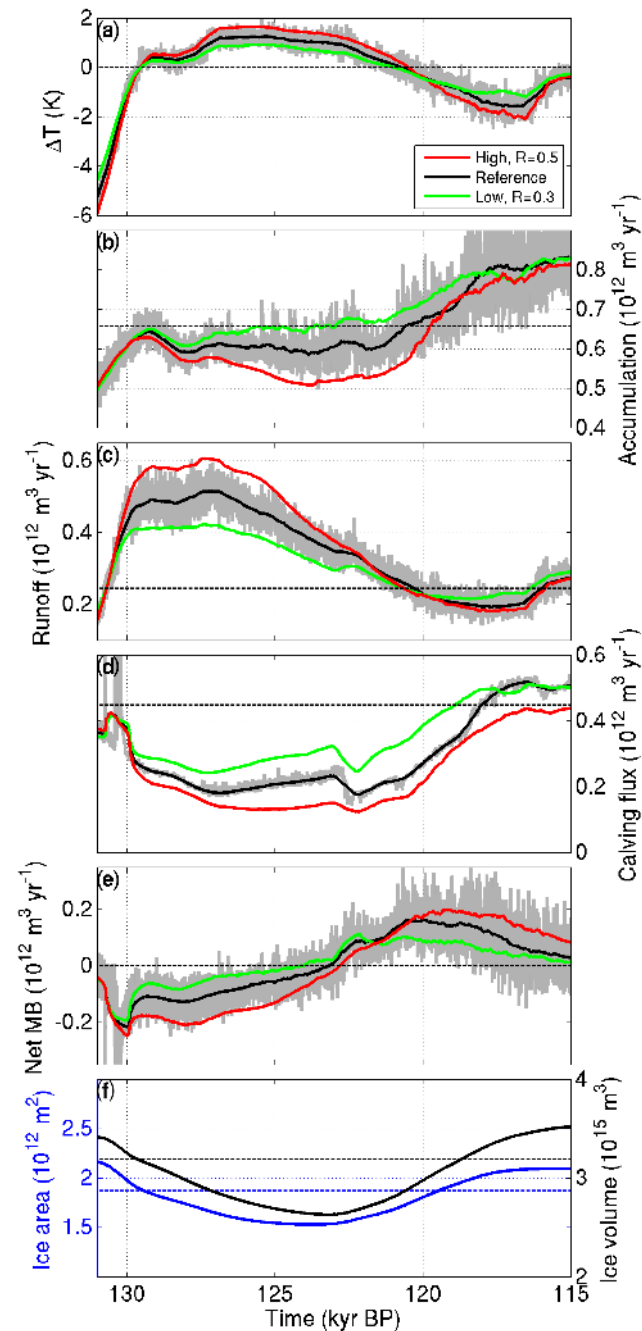
Figure 4. Greenland ice sheet forcing characteristics for the reference run (black) and with higher (red) and lower (green) temperature scaling. Climatic temperature anomaly relative to pre-industrial (a). Accumulation (b) and surface meltwater runoff (c) over grounded ice. Calving flux (d), net mass balance (e), and other mass balance terms (b, c) given in water equivalent. Ice area (blue) and ice volume (black) for the reference run (f). All lines are smoothed with a 400-year running mean except for the grey lines giving the full annual time resolution for the reference run. Horizontal dashed lines give the pre-industrial reference values, except for panel e, where it is the zero line.
