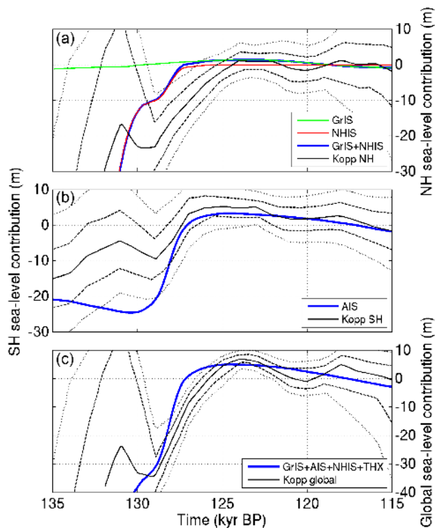
Figure 12. Modelled sea-level contributions from this study (colour lines) compared to probabilistic sea-level reconstructions (black lines) from Kopp et al. (2009) for the NH (a), the SH (b), and globally (c). For the reconstructions, solid lines correspond to the median projection, dashed lines to the 16th and 84th percentiles, and dotted lines to the 2.5th and 97.5th percentiles.
