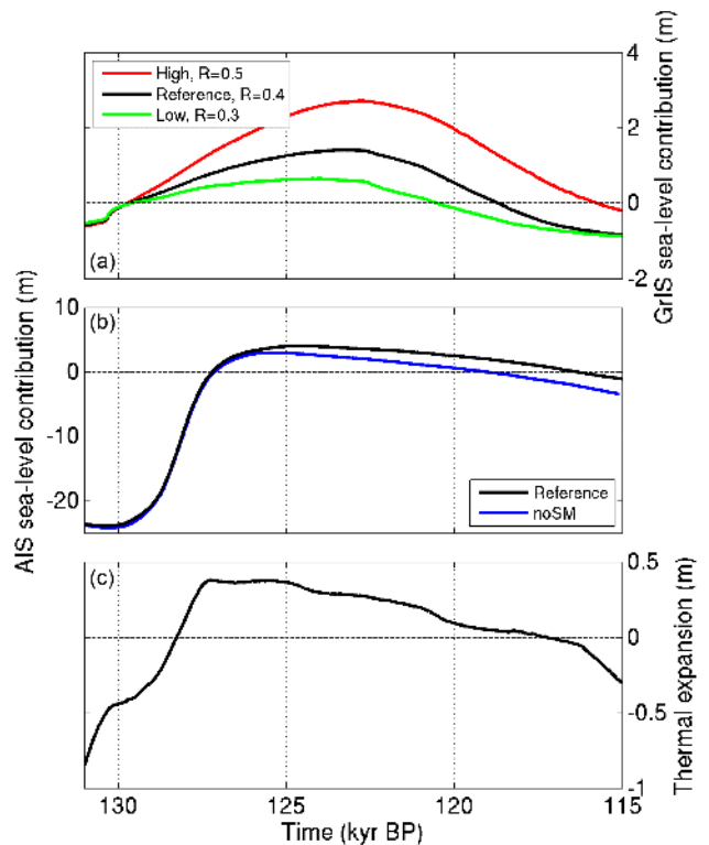
Figure 11. Sea-level contribution from the Greenland ice sheet for the reference run (black) and two sensitivity experiments with higher (red) and lower (green) temperature scaling (a). Sea-level contribution from the Antarctic ice sheet from the reference run (black) and from a sensitivity experiment without sub-shelf melting (blue) (b). Sea-level contribution from oceanic thermal expansion from the reference run (c).
