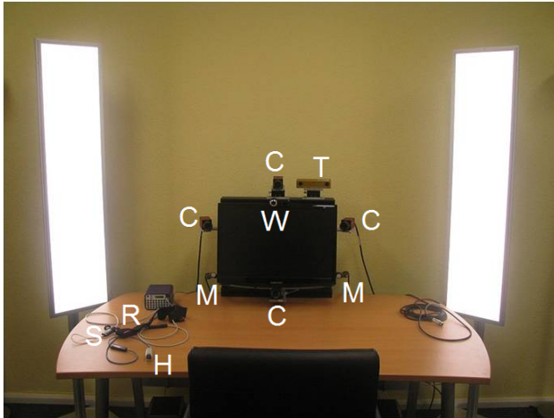
Figure 2: The hardware setting in the subject room. C=High resolution camera, H=Heart beat clip, M=Microphone, R=Respiration belt, S=Skin conductance clip, T=Stereo camera, W=Observation webcam. Not in the picture: Headwear microphone.
